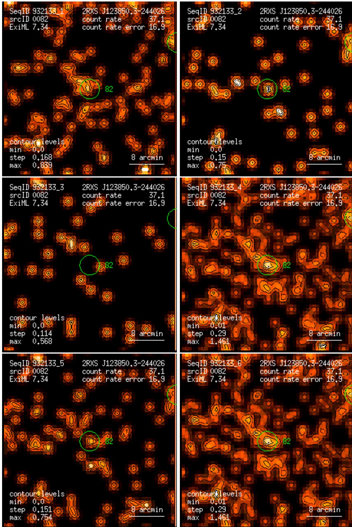
Figure 82: RASS 932133: detection 0082: band rate images, Gaussian filter: (1) PSPC channels 11 – 41, (2) 52 – 90, (3) 91 – 201, (4) 11 – 235, (5) 52 – 201, (6) 11 – 201. Broad band rates in counts/ks. Band rate contour levels in counts/ks/arcmin 2 .
