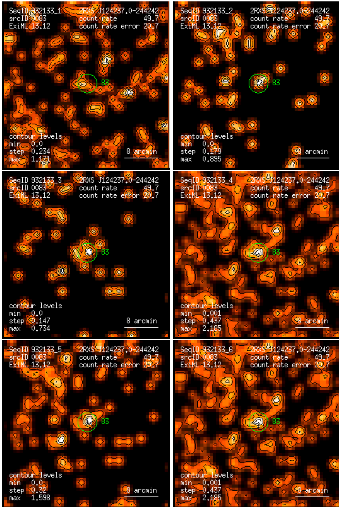
Figure 83: RASS 932133: detection 0083: band rate images, Gaussian filter: (1) PSPC channels 11 – 41, (2) 52 – 90, (3) 91 – 201, (4) 11 – 235, (5) 52 – 201, (6) 11 – 201. Broad band rates in counts/ks. Band rate contour levels in counts/ks/arcmin 2 .
