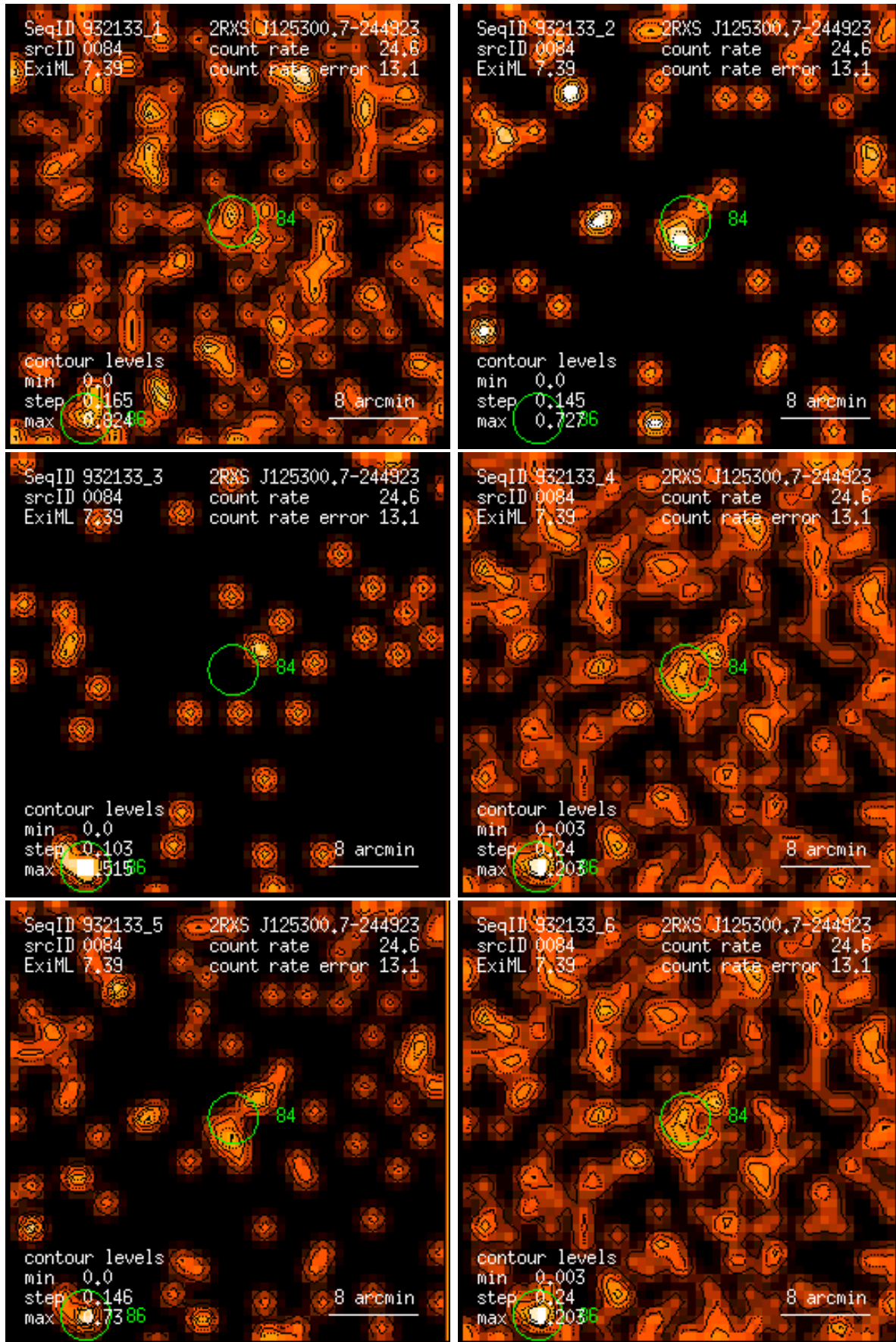
Figure 84: RASS 932133: detection 0084: band rate images, Gaussian filter: (1) PSPC channels 11 – 41, (2) 52 – 90, (3) 91 – 201, (4) 11 – 235, (5) 52 – 201, (6) 11 – 201. Broad band rates in counts/ks. Band rate contour levels in counts/ks/arcmin 2 .
