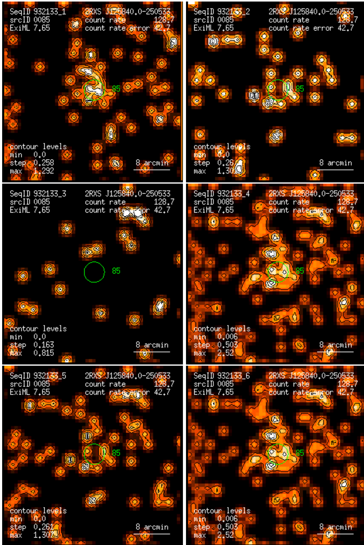
Figure 85: RASS 932133: detection 0085: band rate images, Gaussian filter: (1) PSPC channels 11 – 41, (2) 52 – 90, (3) 91 – 201, (4) 11 – 235, (5) 52 – 201, (6) 11 – 201. Broad band rates in counts/ks. Band rate contour levels in counts/ks/arcmin 2 .
