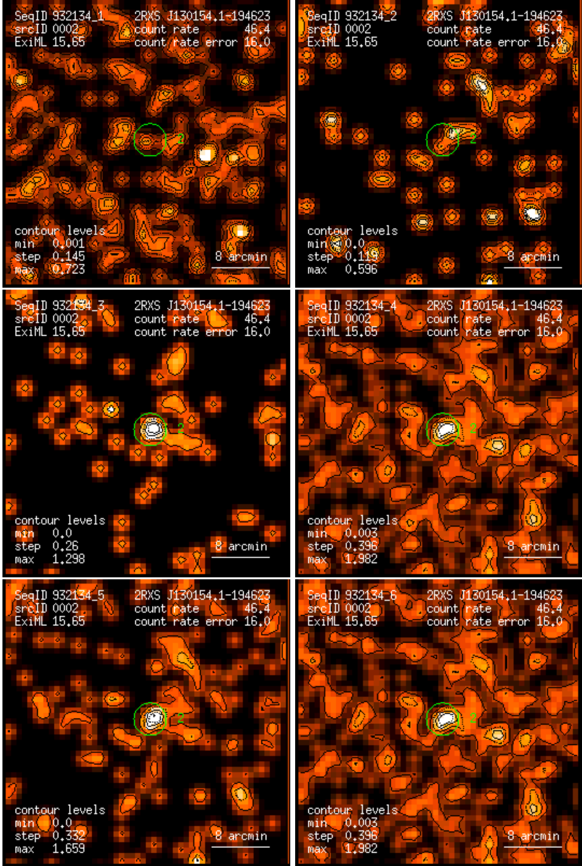
Figure 2: RASS 932134: detection 0002: band rate images, Gaussian filter: (1) PSPC channels 11 – 41, (2) 52 – 90, (3) 91 – 201, (4) 11 – 235, (5) 52 – 201, (6) 11 – 201. Broad band rates in counts/ks. Band rate contour levels in counts/ks/arcmin 2 .
