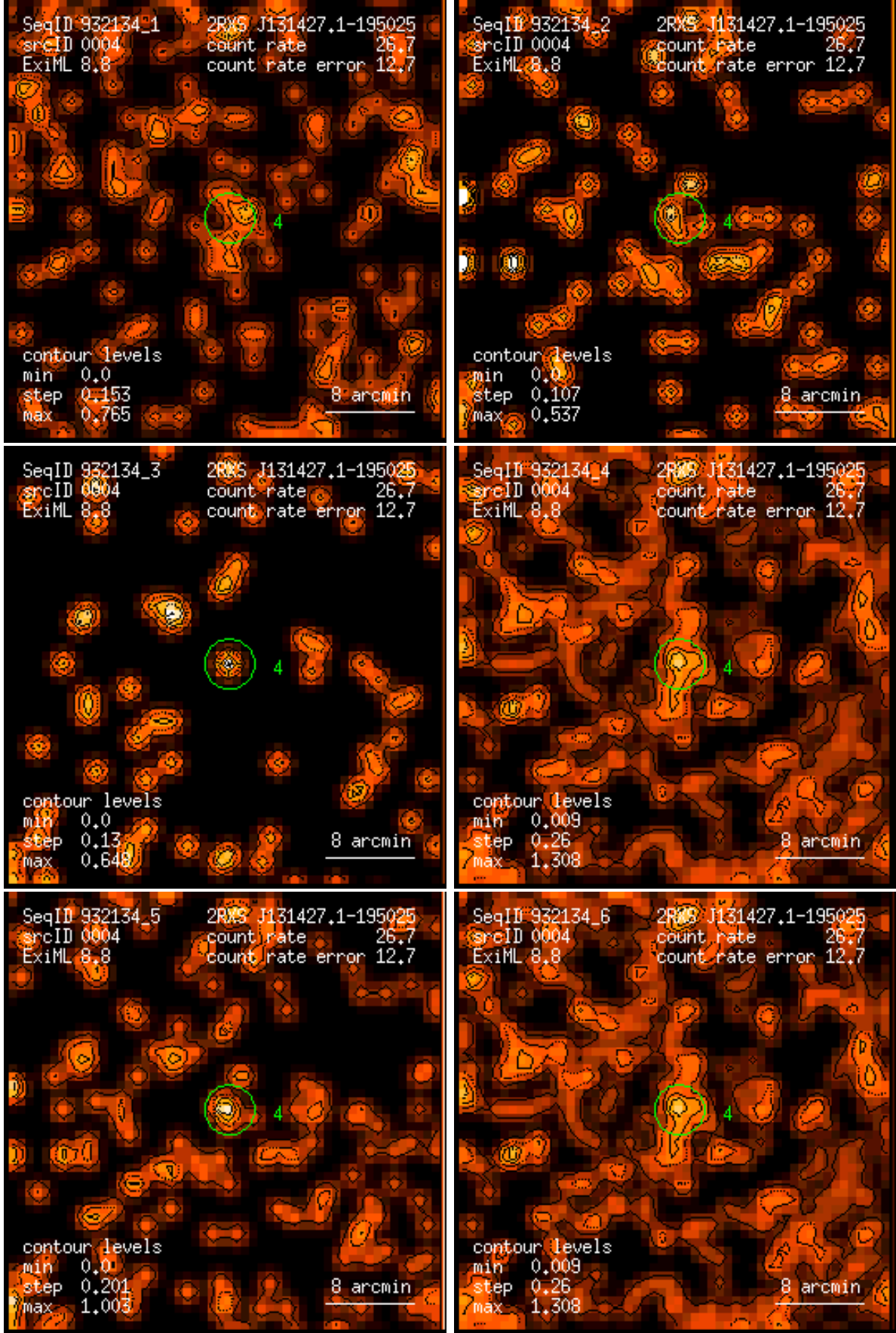
Figure 4: RASS 932134: detection 0004: band rate images, Gaussian filter: (1) PSPC channels 11 – 41, (2) 52 – 90, (3) 91 – 201, (4) 11 – 235, (5) 52 – 201, (6) 11 – 201. Broad band rates in counts/ks. Band rate contour levels in counts/ks/arcmin 2 .
