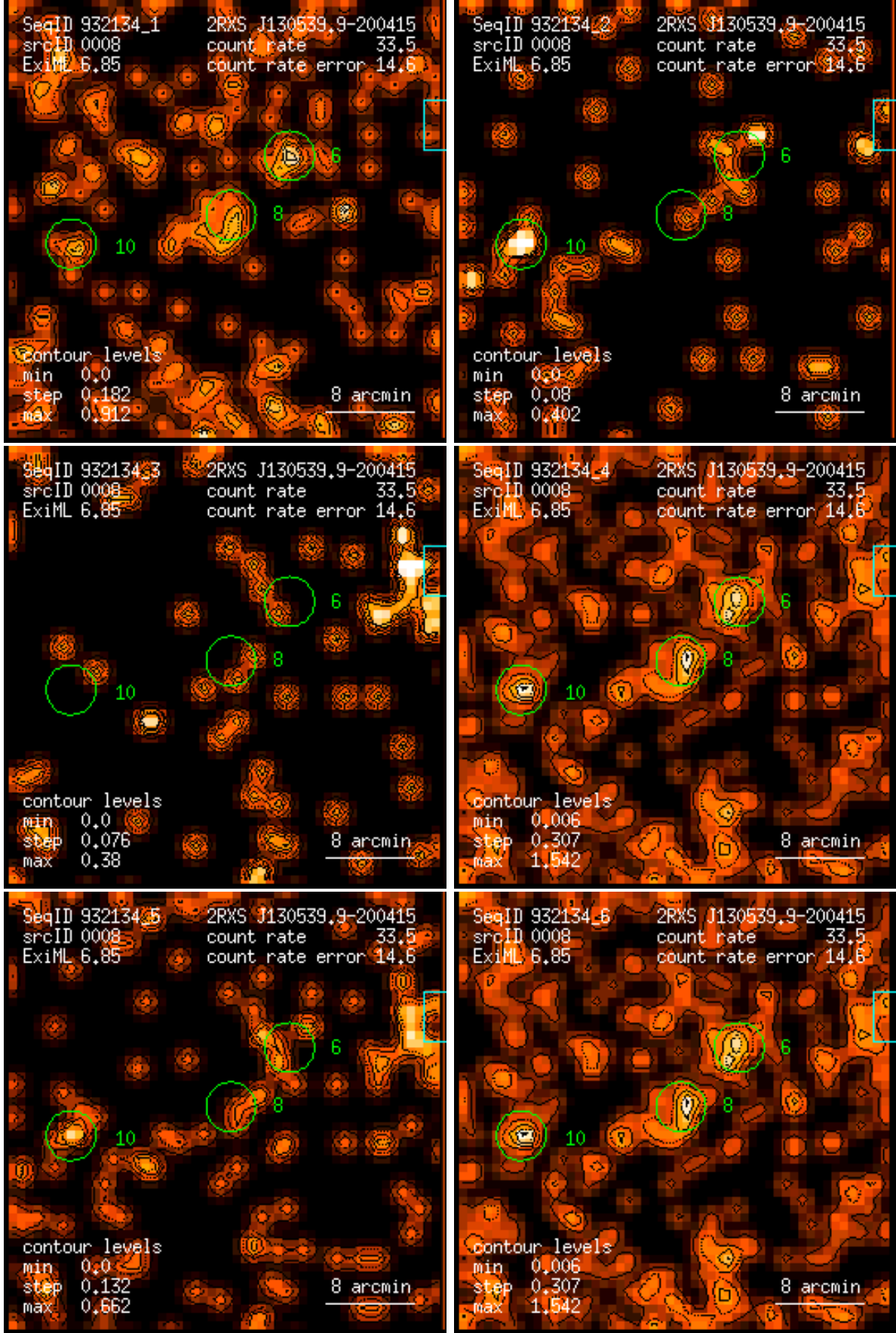
Figure 8: RASS 932134: detection 0008: band rate images, Gaussian filter: (1) PSPC channels 11 – 41, (2) 52 – 90, (3) 91 – 201, (4) 11 – 235, (5) 52 – 201, (6) 11 – 201. Broad band rates in counts/ks. Band rate contour levels in counts/ks/arcmin 2 .
