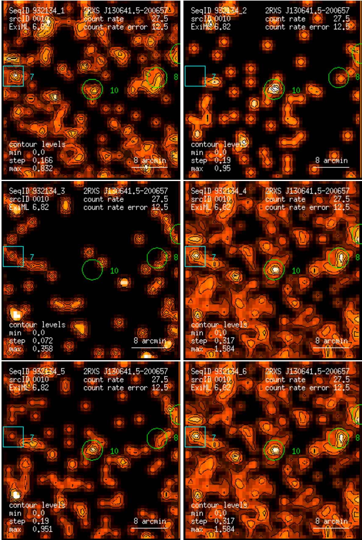
Figure 10: RASS 932134: detection 0010: band rate images, Gaussian filter: (1) PSPC channels 11 – 41, (2) 52 – 90, (3) 91 – 201, (4) 11 – 235, (5) 52 – 201, (6) 11 – 201. Broad band rates in counts/ks. Band rate contour levels in counts/ks/arcmin 2 .
