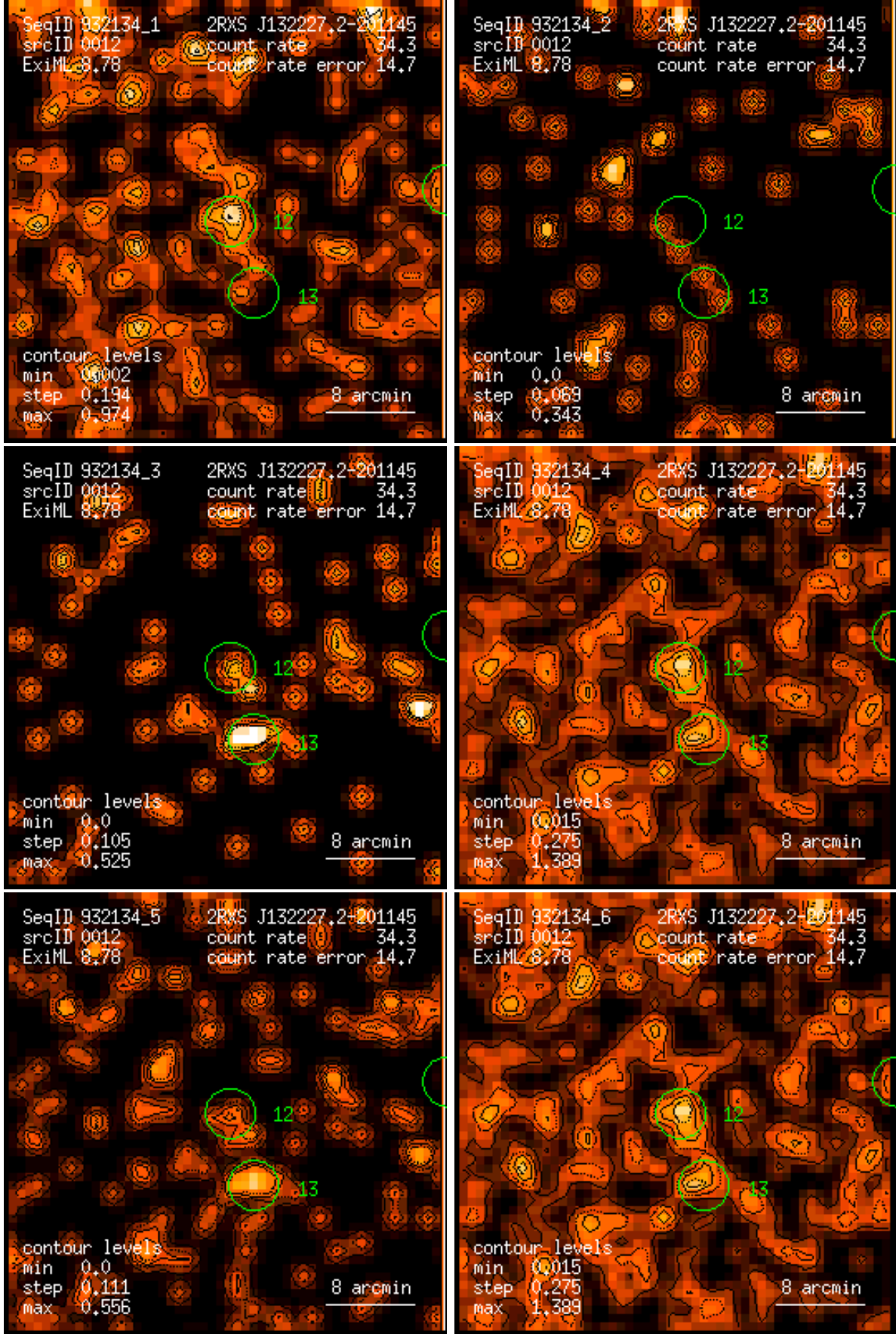
Figure 12: RASS 932134: detection 0012: band rate images, Gaussian filter: (1) PSPC channels 11 – 41, (2) 52 – 90, (3) 91 – 201, (4) 11 – 235, (5) 52 – 201, (6) 11 – 201. Broad band rates in counts/ks. Band rate contour levels in counts/ks/arcmin 2 .
