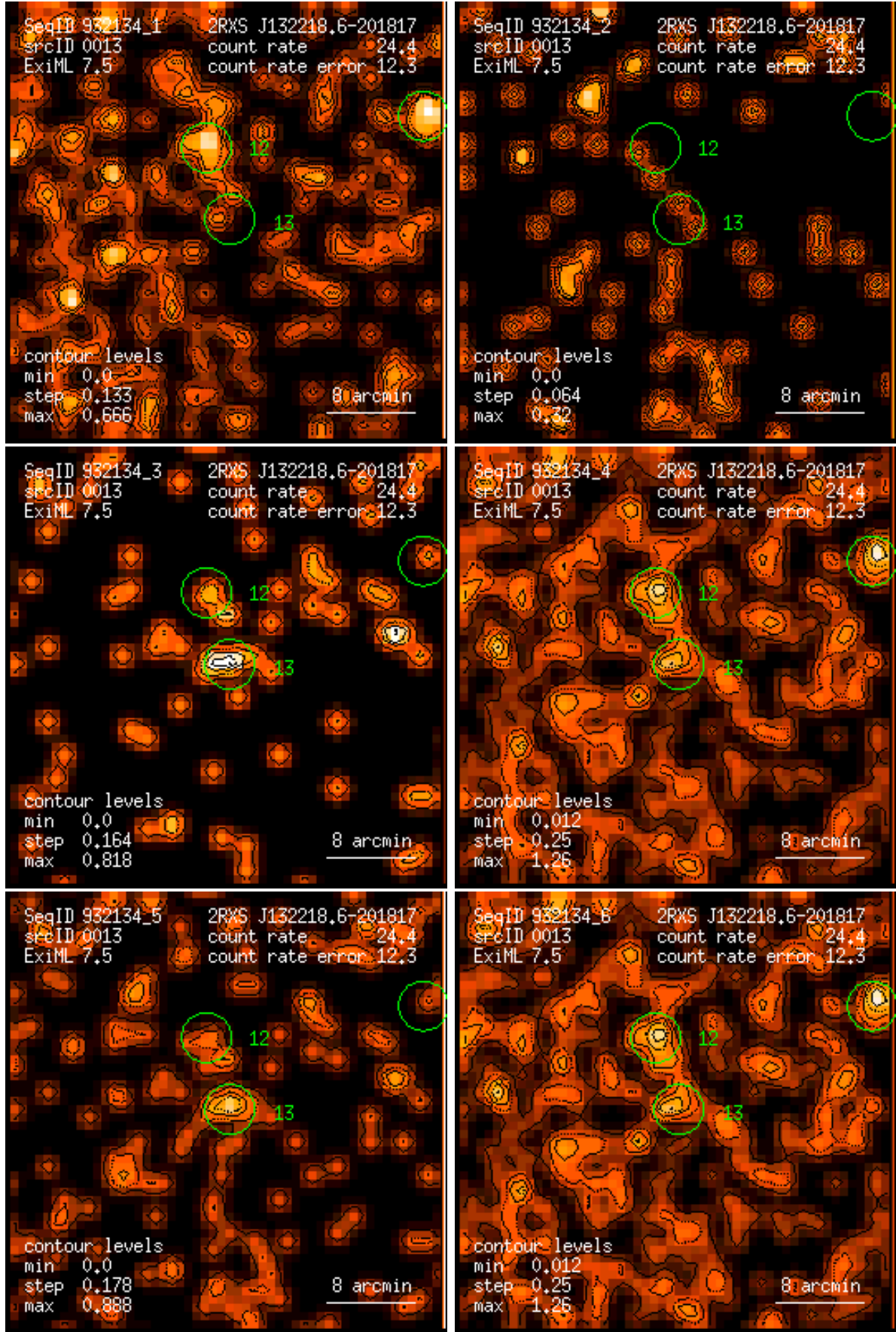
Figure 13: RASS 932134: detection 0013: band rate images, Gaussian filter: (1) PSPC channels 11 – 41, (2) 52 – 90, (3) 91 – 201, (4) 11 – 235, (5) 52 – 201, (6) 11 – 201. Broad band rates in counts/ks. Band rate contour levels in counts/ks/arcmin 2 .
