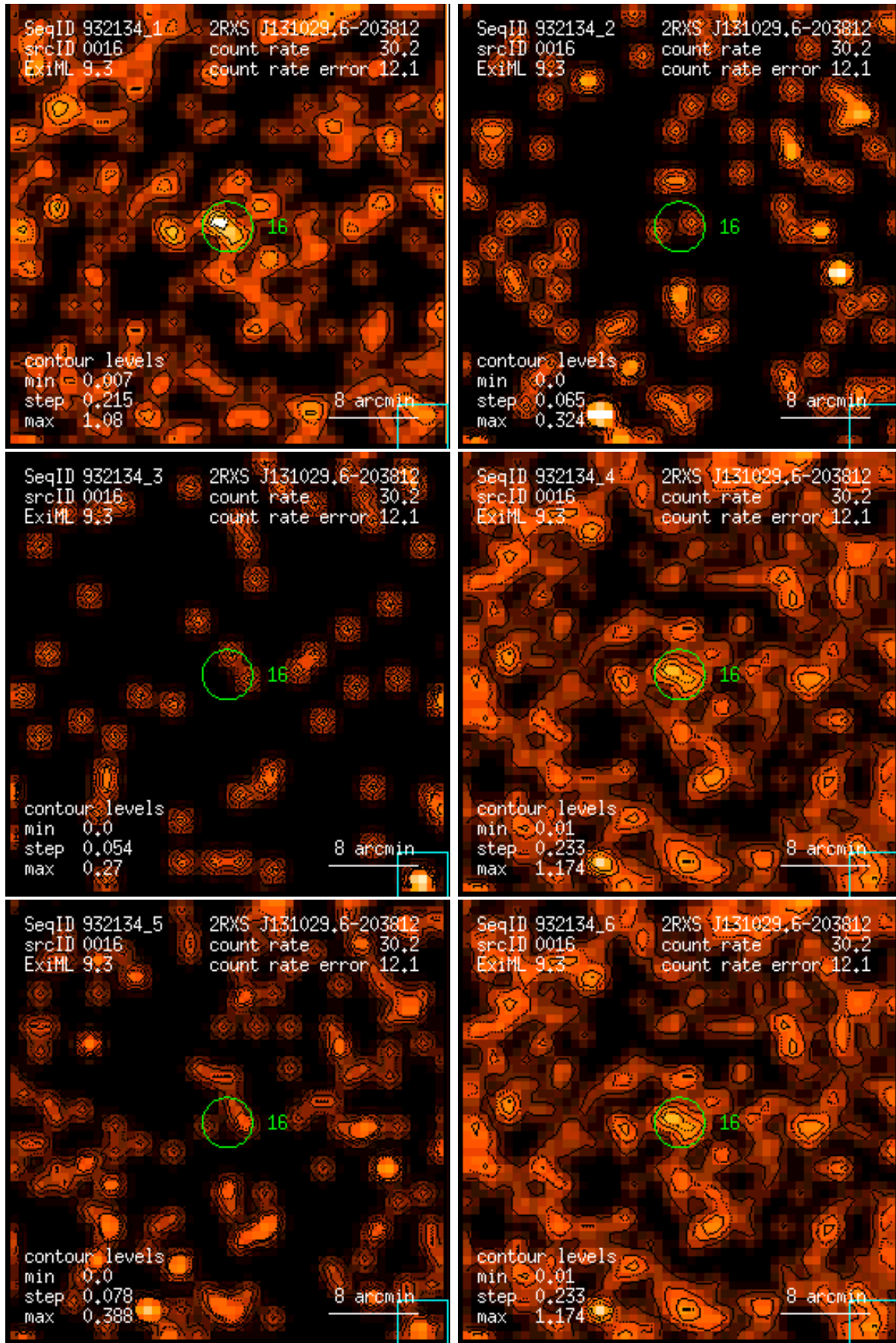
Figure 16: RASS 932134: detection 0016: band rate images, Gaussian filter: (1) PSPC channels 11 – 41, (2) 52 – 90, (3) 91 – 201, (4) 11 – 235, (5) 52 – 201, (6) 11 – 201. Broad band rates in counts/ks. Band rate contour levels in counts/ks/arcmin 2 .
