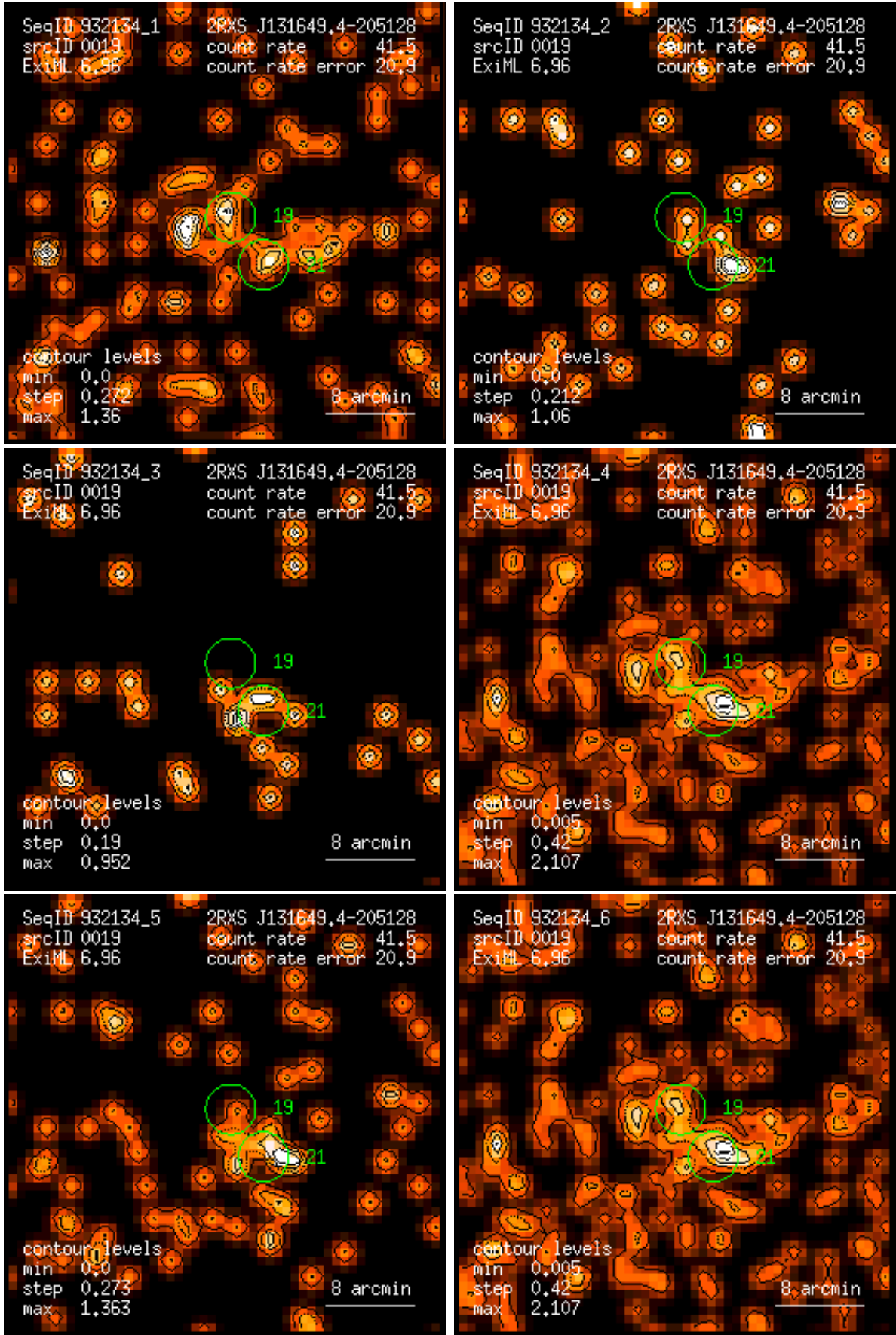
Figure 19: RASS 932134: detection 0019: band rate images, Gaussian filter: (1) PSPC channels 11 – 41, (2) 52 – 90, (3) 91 – 201, (4) 11 – 235, (5) 52 – 201, (6) 11 – 201. Broad band rates in counts/ks. Band rate contour levels in counts/ks/arcmin 2 .
