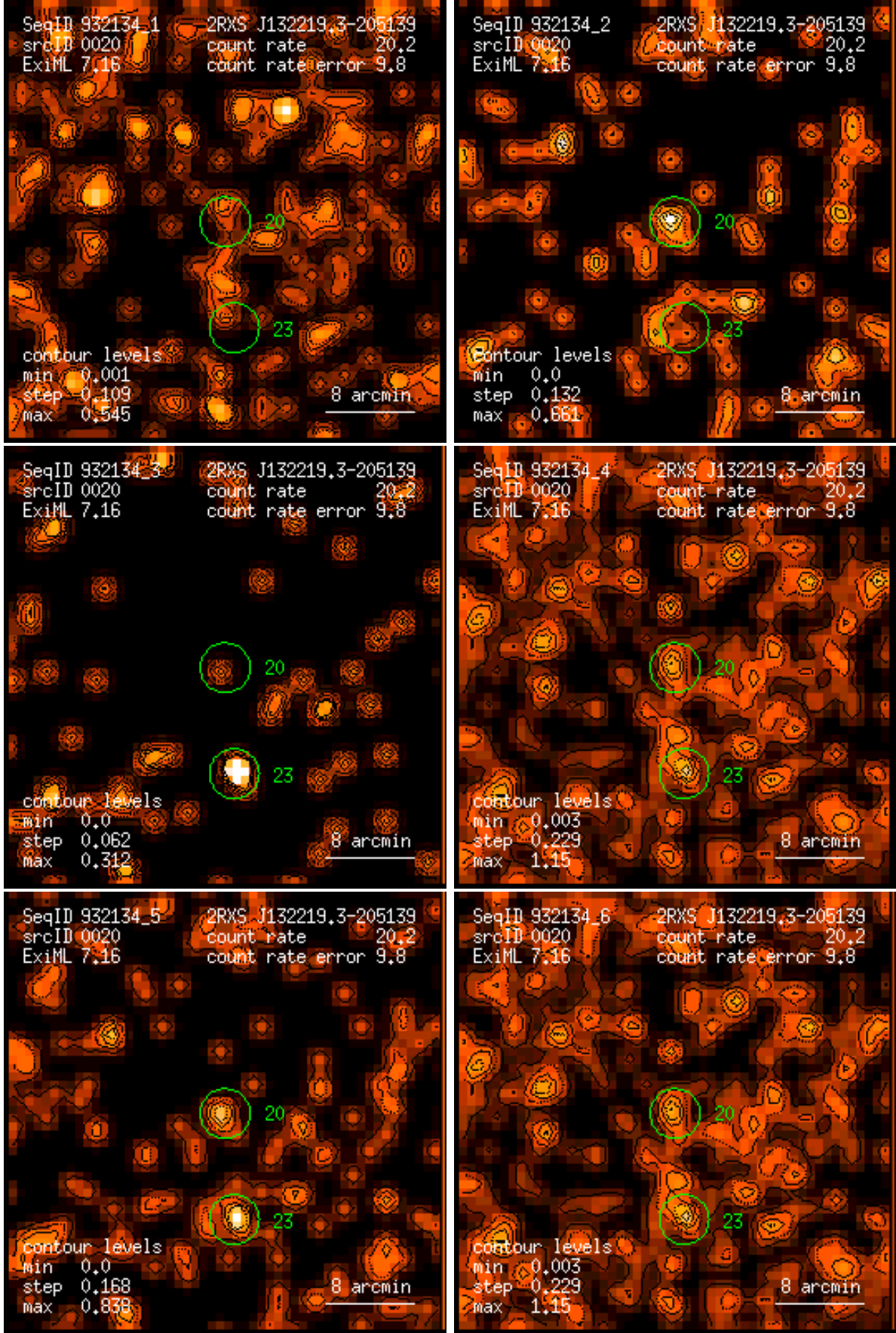
Figure 20: RASS 932134: detection 0020: band rate images, Gaussian filter: (1) PSPC channels 11 – 41, (2) 52 – 90, (3) 91 – 201, (4) 11 – 235, (5) 52 – 201, (6) 11 – 201. Broad band rates in counts/ks. Band rate contour levels in counts/ks/arcmin 2 .
