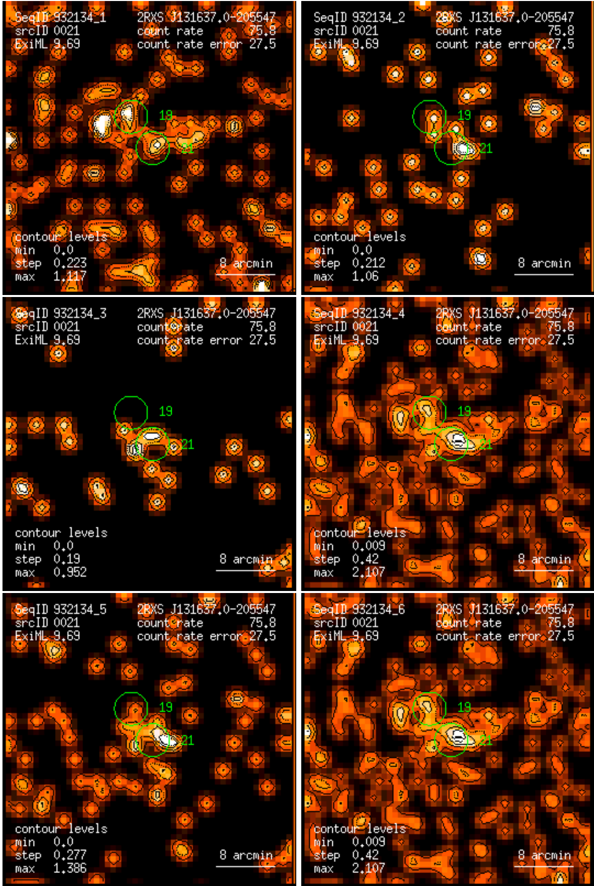
Figure 21: RASS 932134: detection 0021: band rate images, Gaussian filter: (1) PSPC channels 11 – 41, (2) 52 – 90, (3) 91 – 201, (4) 11 – 235, (5) 52 – 201, (6) 11 – 201. Broad band rates in counts/ks. Band rate contour levels in counts/ks/arcmin 2 .
