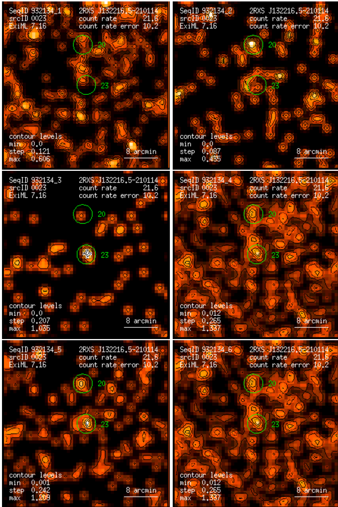
Figure 23: RASS 932134: detection 0023: band rate images, Gaussian filter: (1) PSPC channels 11 – 41, (2) 52 – 90, (3) 91 – 201, (4) 11 – 235, (5) 52 – 201, (6) 11 – 201. Broad band rates in counts/ks. Band rate contour levels in counts/ks/arcmin 2 .
