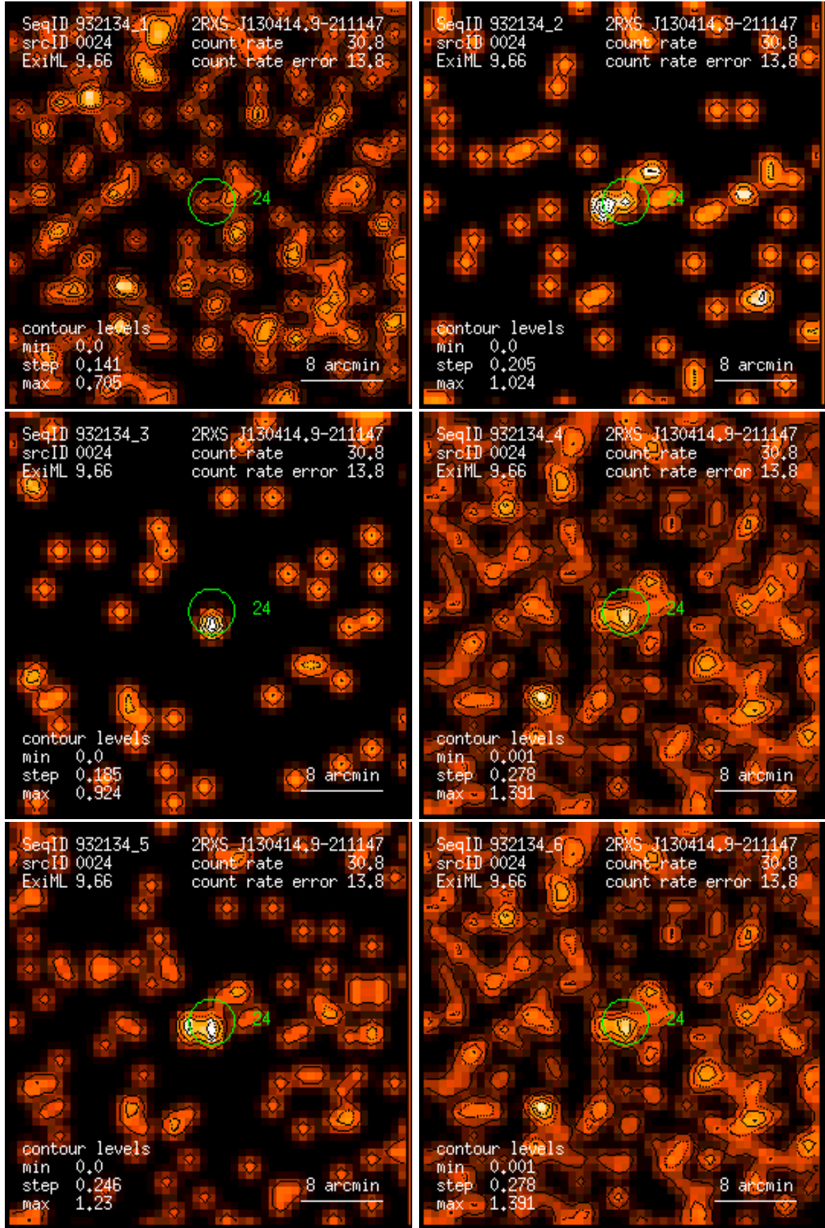
Figure 24: RASS 932134: detection 0024: band rate images, Gaussian filter: (1) PSPC channels 11 – 41, (2) 52 – 90, (3) 91 – 201, (4) 11 – 235, (5) 52 – 201, (6) 11 – 201. Broad band rates in counts/ks. Band rate contour levels in counts/ks/arcmin 2 .
