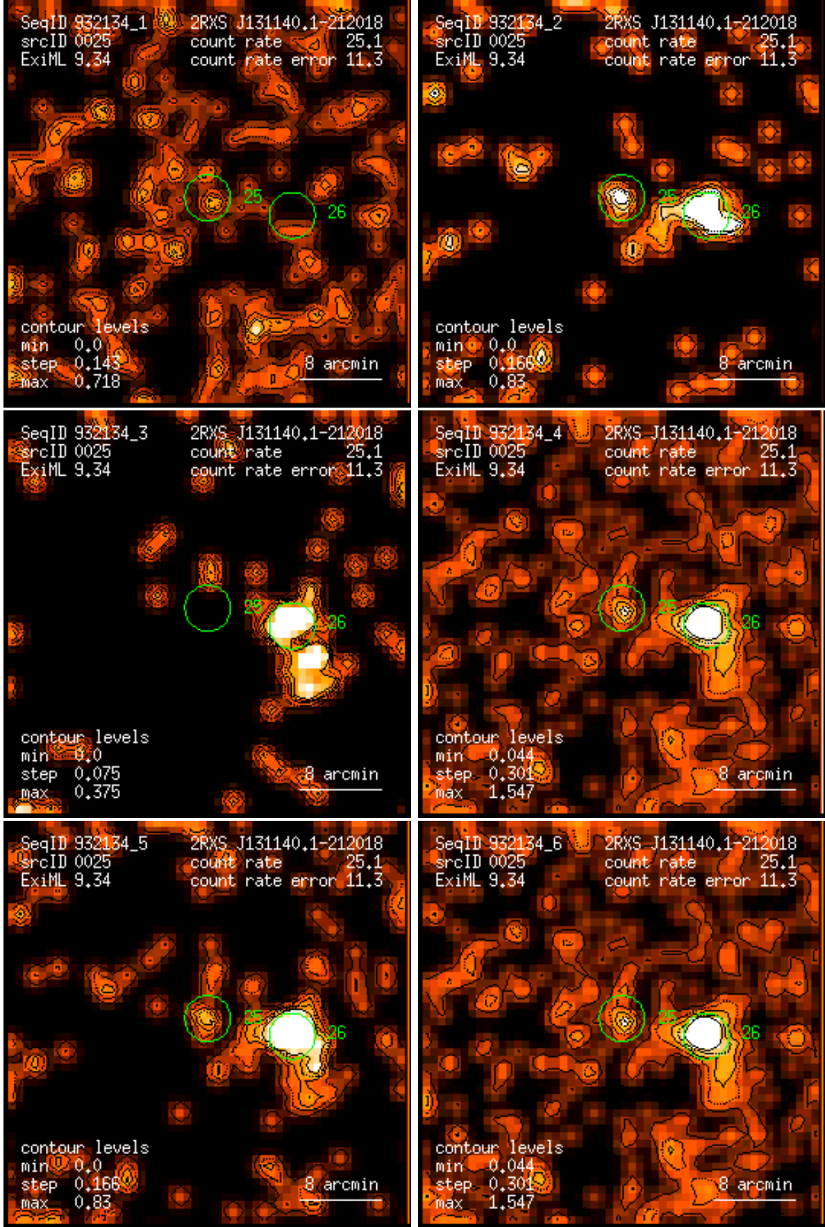
Figure 25: RASS 932134: detection 0025: band rate images, Gaussian filter: (1) PSPC channels 11 – 41, (2) 52 – 90, (3) 91 – 201, (4) 11 – 235, (5) 52 – 201, (6) 11 – 201. Broad band rates in counts/ks. Band rate contour levels in counts/ks/arcmin 2 .
