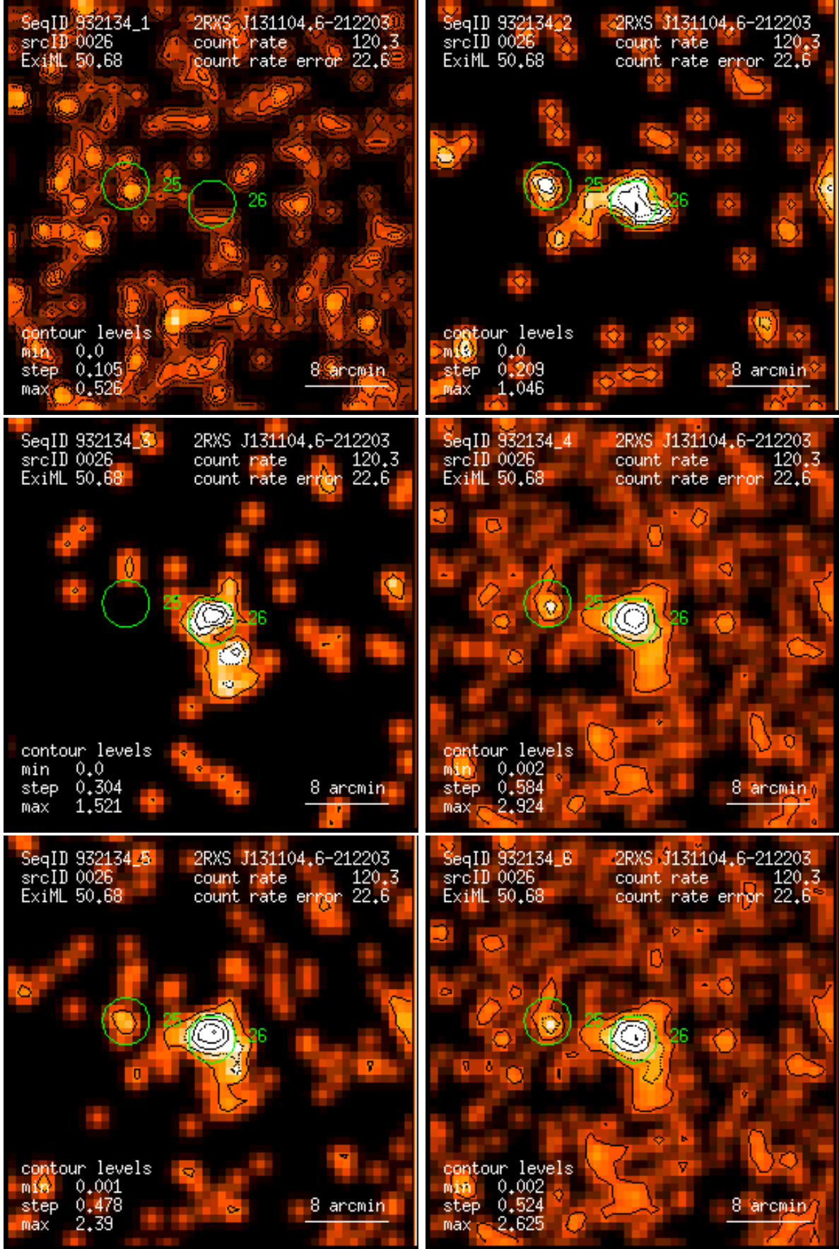
Figure 26: RASS 932134: detection 0026: band rate images, Gaussian filter: (1) PSPC channels 11 – 41, (2) 52 – 90, (3) 91 – 201, (4) 11 – 235, (5) 52 – 201, (6) 11 – 201. Broad band rates in counts/ks. Band rate contour levels in counts/ks/arcmin 2 .
