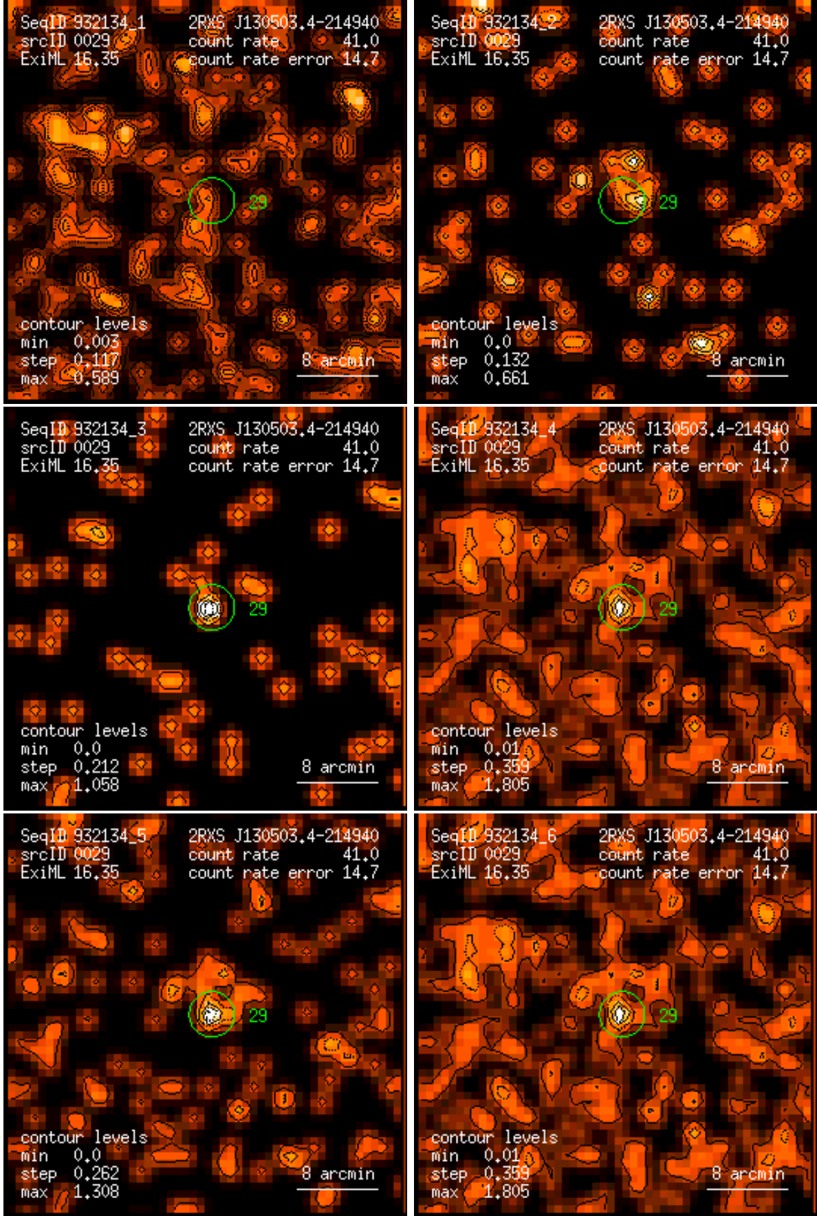
Figure 29: RASS 932134: detection 0029: band rate images, Gaussian filter: (1) PSPC channels 11 – 41, (2) 52 – 90, (3) 91 – 201, (4) 11 – 235, (5) 52 – 201, (6) 11 – 201. Broad band rates in counts/ks. Band rate contour levels in counts/ks/arcmin 2 .
