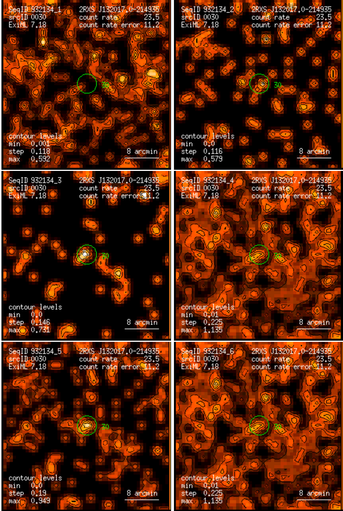
Figure 30: RASS 932134: detection 0030: band rate images, Gaussian filter: (1) PSPC channels 11 – 41, (2) 52 – 90, (3) 91 – 201, (4) 11 – 235, (5) 52 – 201, (6) 11 – 201. Broad band rates in counts/ks. Band rate contour levels in counts/ks/arcmin 2 .
