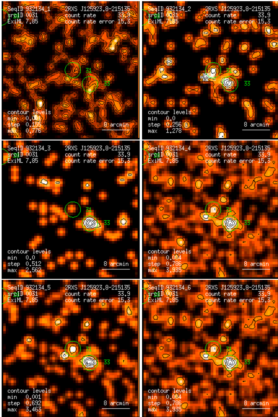
Figure 31: RASS 932134: detection 0031: band rate images, Gaussian filter: (1) PSPC channels 11 – 41, (2) 52 – 90, (3) 91 – 201, (4) 11 – 235, (5) 52 – 201, (6) 11 – 201. Broad band rates in counts/ks. Band rate contour levels in counts/ks/arcmin 2 .
