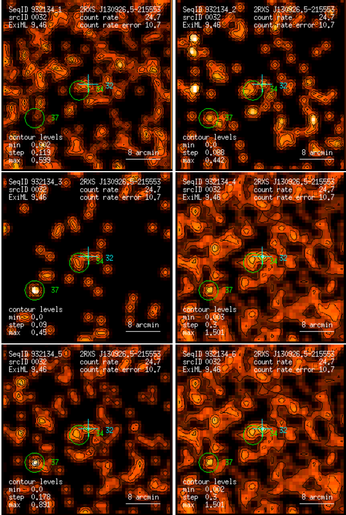
Figure 32: RASS 932134: detection 0032: band rate images, Gaussian filter: (1) PSPC channels 11 – 41, (2) 52 – 90, (3) 91 – 201, (4) 11 – 235, (5) 52 – 201, (6) 11 – 201. Broad band rates in counts/ks. Band rate contour levels in counts/ks/arcmin 2 .
