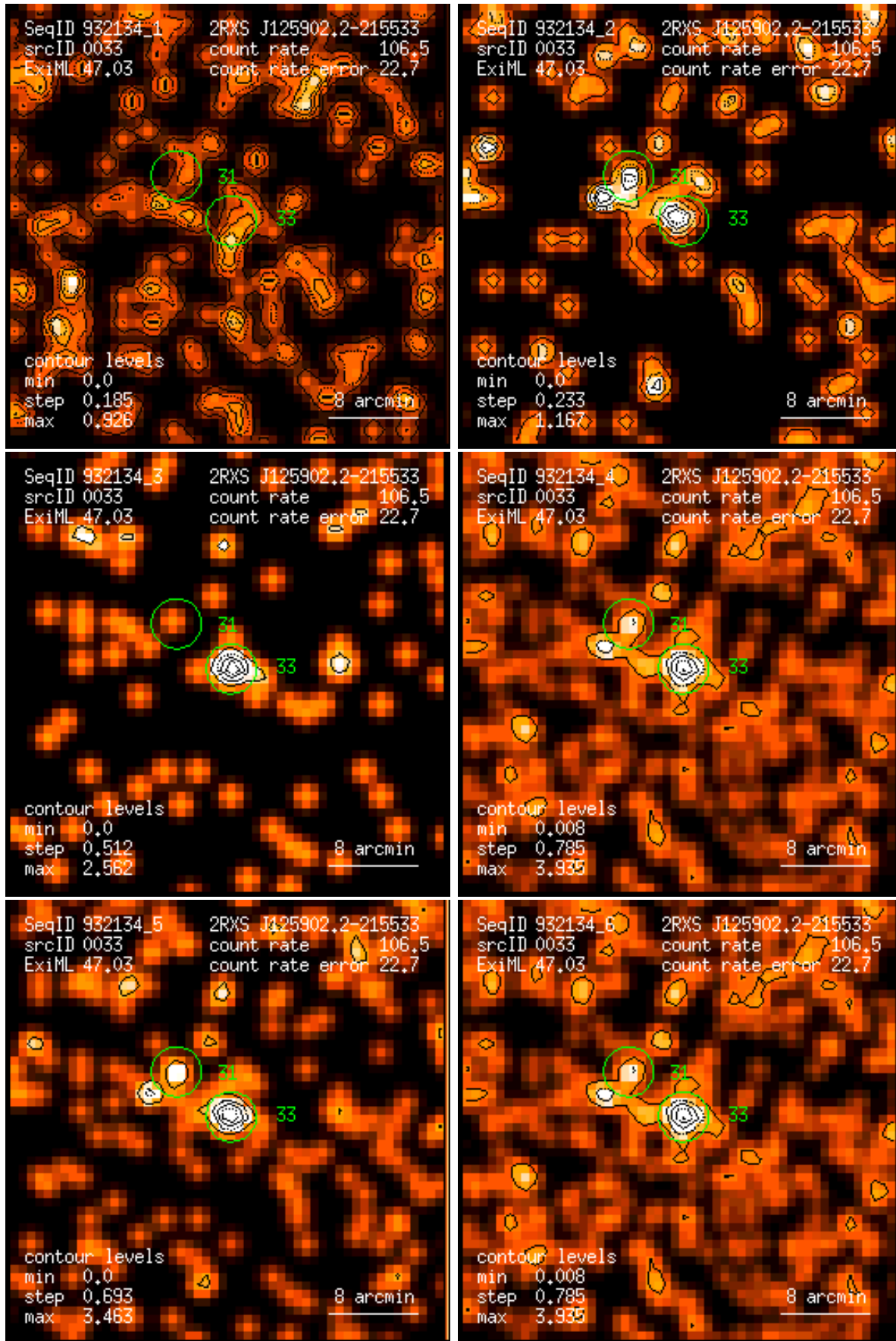
Figure 33: RASS 932134: detection 0033: band rate images, Gaussian filter: (1) PSPC channels 11 – 41, (2) 52 – 90, (3) 91 – 201, (4) 11 – 235, (5) 52 – 201, (6) 11 – 201. Broad band rates in counts/ks. Band rate contour levels in counts/ks/arcmin 2 .
