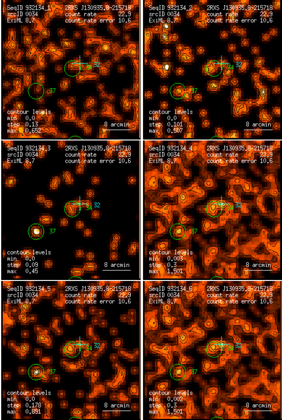
Figure 34: RASS 932134: detection 0034: band rate images, Gaussian filter: (1) PSPC channels 11 – 41, (2) 52 – 90, (3) 91 – 201, (4) 11 – 235, (5) 52 – 201, (6) 11 – 201. Broad band rates in counts/ks. Band rate contour levels in counts/ks/arcmin 2 .
