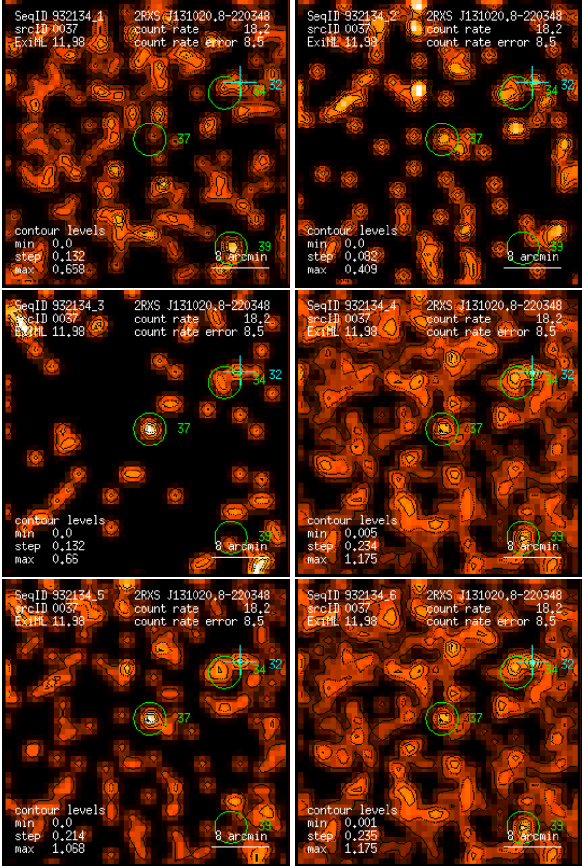
Figure 37: RASS 932134: detection 0037: band rate images, Gaussian filter: (1) PSPC channels 11 – 41, (2) 52 – 90, (3) 91 – 201, (4) 11 – 235, (5) 52 – 201, (6) 11 – 201. Broad band rates in counts/ks. Band rate contour levels in counts/ks/arcmin 2 .
