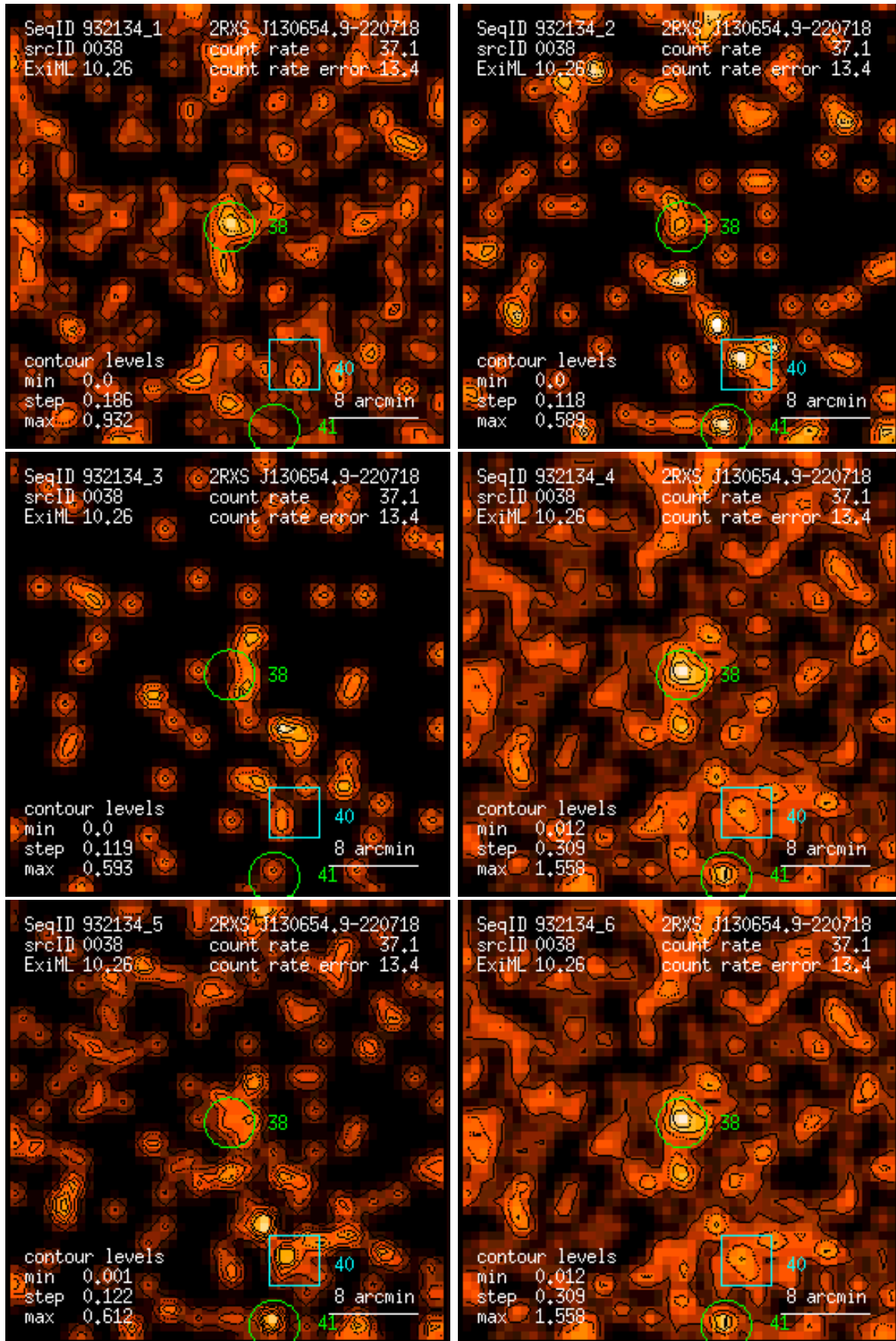
Figure 38: RASS 932134: detection 0038: band rate images, Gaussian filter: (1) PSPC channels 11 – 41, (2) 52 – 90, (3) 91 – 201, (4) 11 – 235, (5) 52 – 201, (6) 11 – 201. Broad band rates in counts/ks. Band rate contour levels in counts/ks/arcmin 2 .
