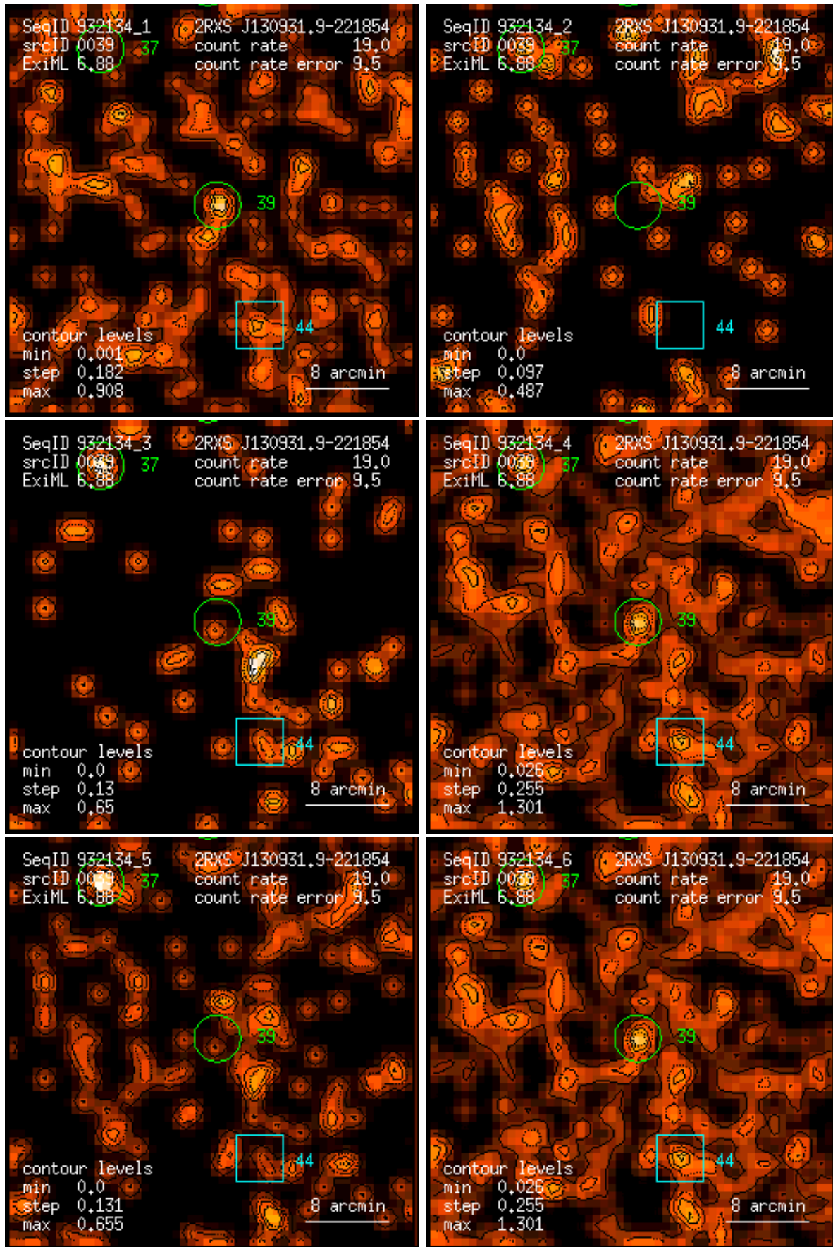
Figure 39: RASS 932134: detection 0039: band rate images, Gaussian filter: (1) PSPC channels 11 – 41, (2) 52 – 90, (3) 91 – 201, (4) 11 – 235, (5) 52 – 201, (6) 11 – 201. Broad band rates in counts/ks. Band rate contour levels in counts/ks/arcmin 2 .
