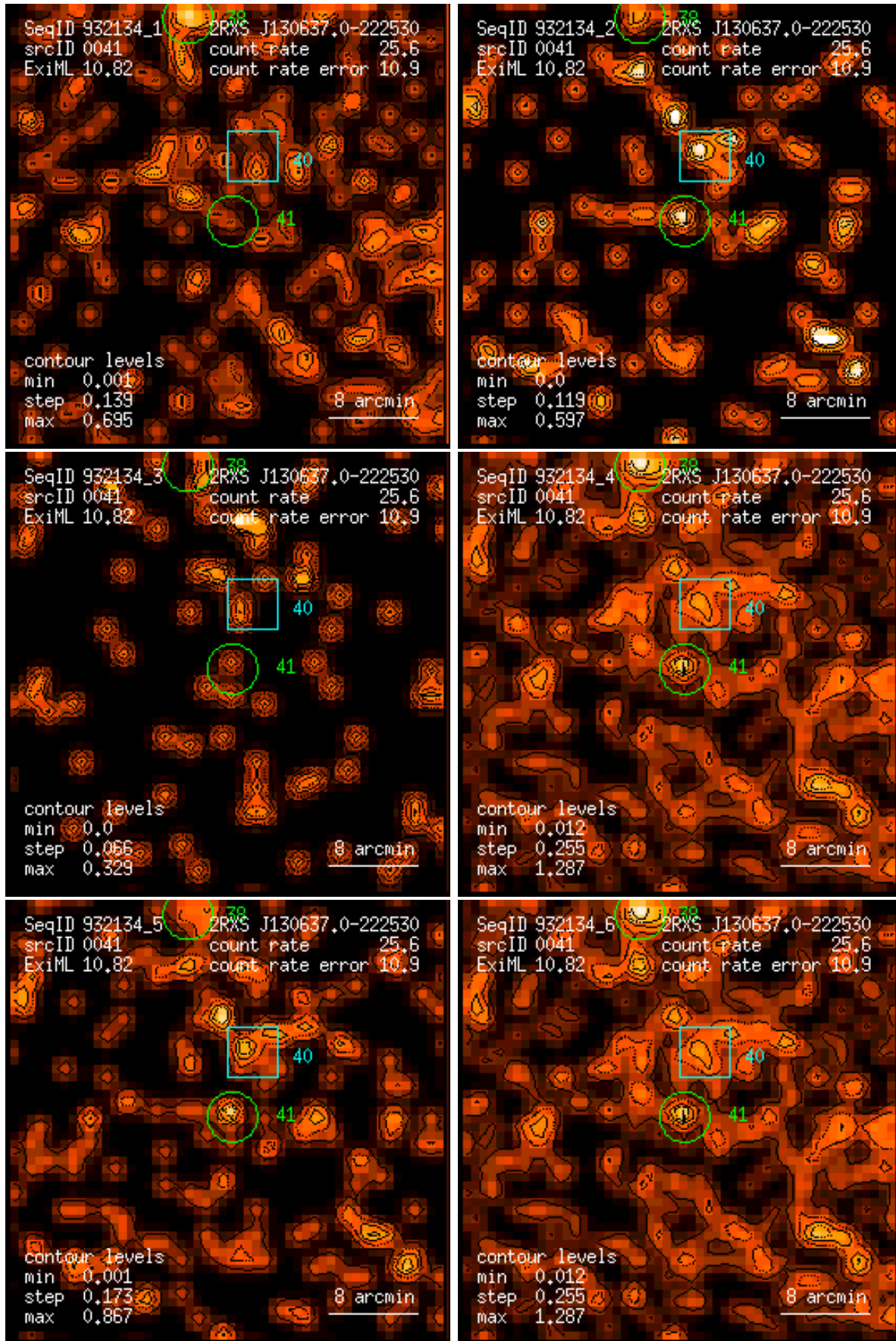
Figure 41: RASS 932134: detection 0041: band rate images, Gaussian filter: (1) PSPC channels 11 – 41, (2) 52 – 90, (3) 91 – 201, (4) 11 – 235, (5) 52 – 201, (6) 11 – 201. Broad band rates in counts/ks. Band rate contour levels in counts/ks/arcmin 2 .
