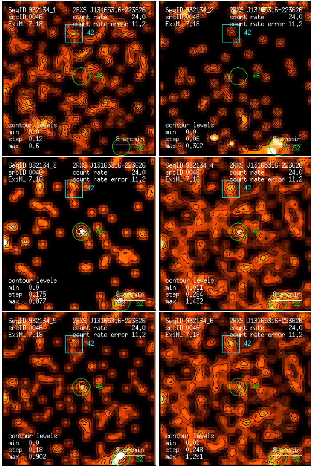
Figure 46: RASS 932134: detection 0046: band rate images, Gaussian filter: (1) PSPC channels 11 – 41, (2) 52 – 90, (3) 91 – 201, (4) 11 – 235, (5) 52 – 201, (6) 11 – 201. Broad band rates in counts/ks. Band rate contour levels in counts/ks/arcmin 2 .
