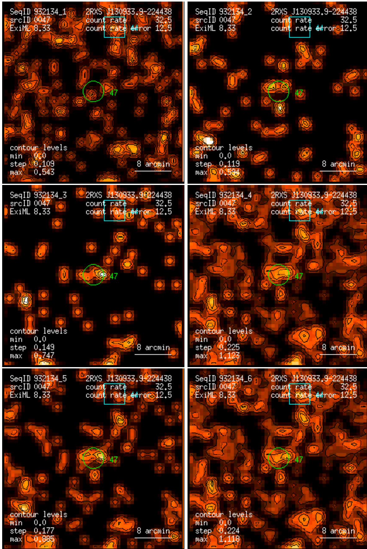
Figure 47: RASS 932134: detection 0047: band rate images, Gaussian filter: (1) PSPC channels 11 – 41, (2) 52 – 90, (3) 91 – 201, (4) 11 – 235, (5) 52 – 201, (6) 11 – 201. Broad band rates in counts/ks. Band rate contour levels in counts/ks/arcmin 2 .
