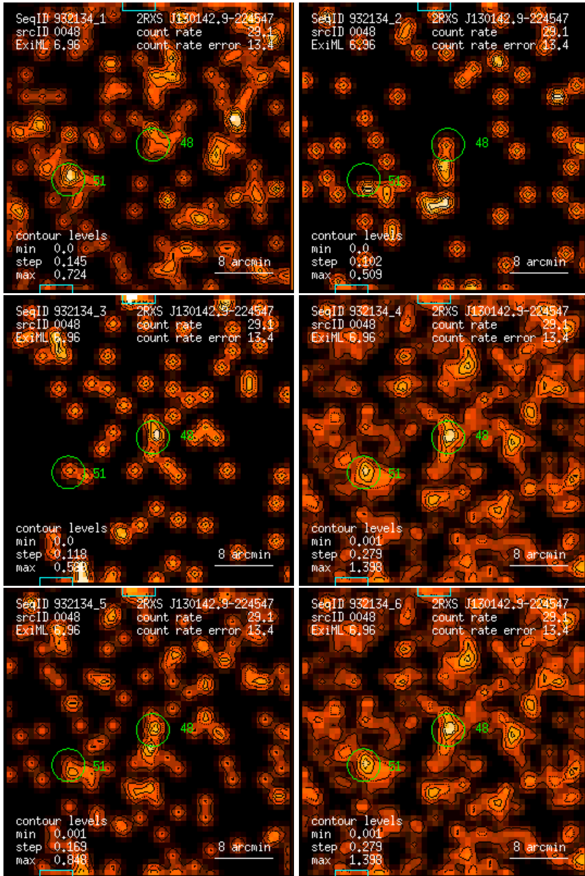
Figure 48: RASS 932134: detection 0048: band rate images, Gaussian filter: (1) PSPC channels 11 – 41, (2) 52 – 90, (3) 91 – 201, (4) 11 – 235, (5) 52 – 201, (6) 11 – 201. Broad band rates in counts/ks. Band rate contour levels in counts/ks/arcmin 2 .
