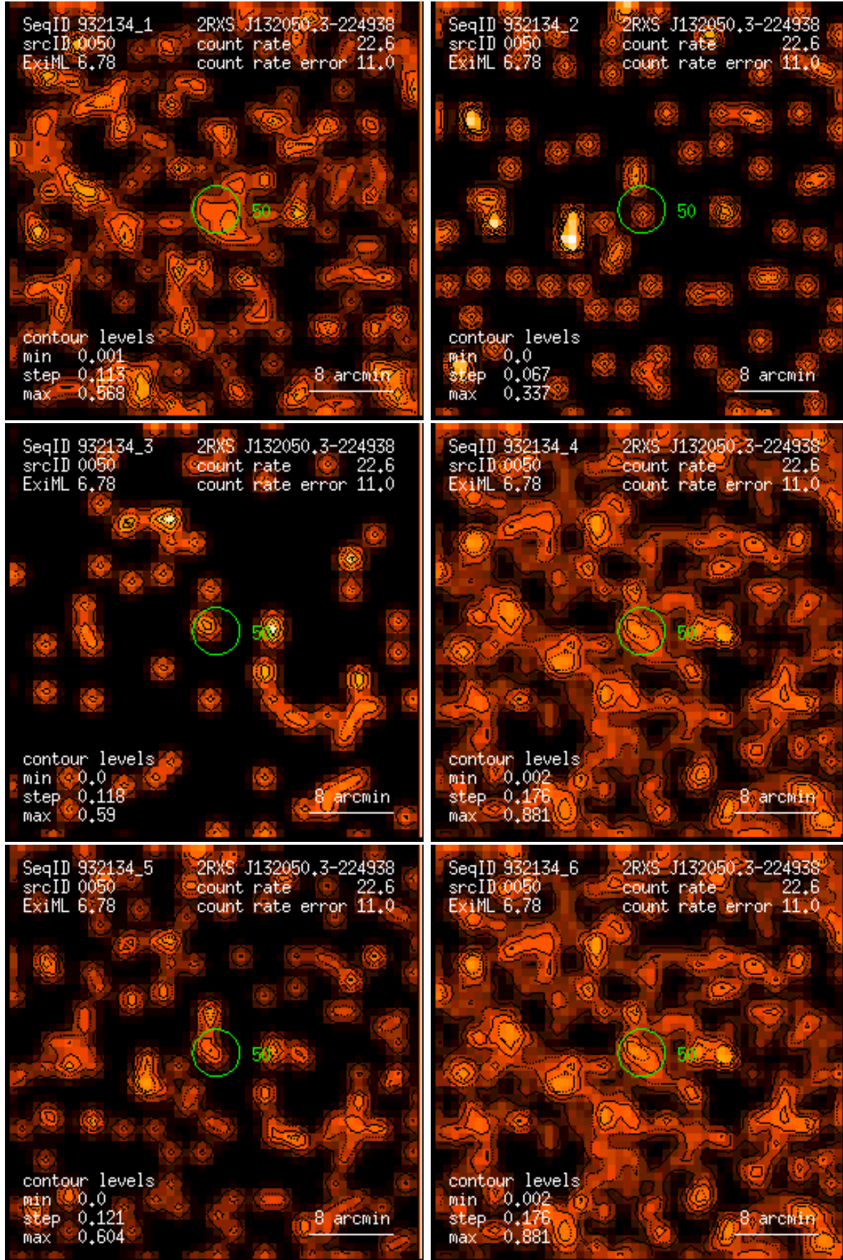
Figure 50: RASS 932134: detection 0050: band rate images, Gaussian filter: (1) PSPC channels 11 – 41, (2) 52 – 90, (3) 91 – 201, (4) 11 – 235, (5) 52 – 201, (6) 11 – 201. Broad band rates in counts/ks. Band rate contour levels in counts/ks/arcmin 2 .
