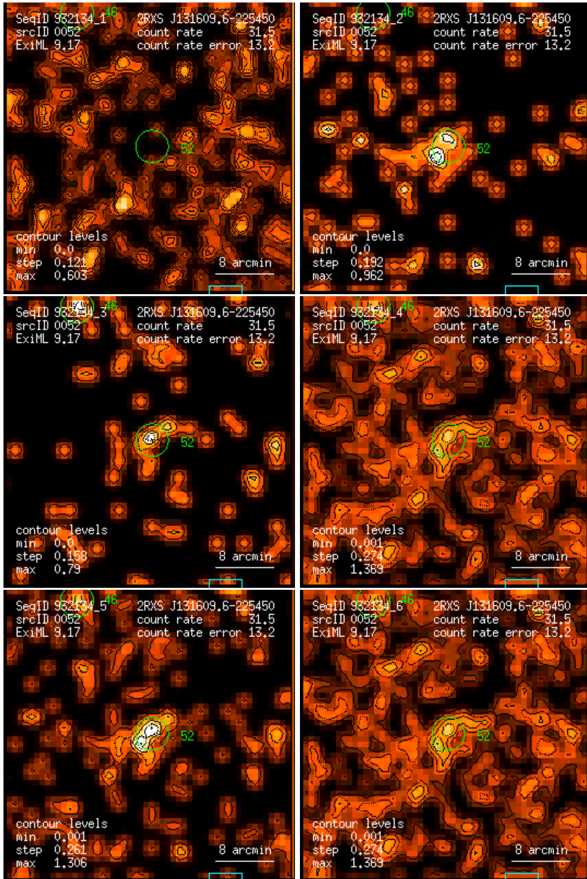
Figure 52: RASS 932134: detection 0052: band rate images, Gaussian filter: (1) PSPP channels 11 – 41, (2) 52 – 90, (3) 91 – 201, (4) 11 – 235, (5) 52 – 201, (6) 11 – 201. Broad band rates in counts/ks. Band rate contour levels in counts/ks/arcmin 2 .
