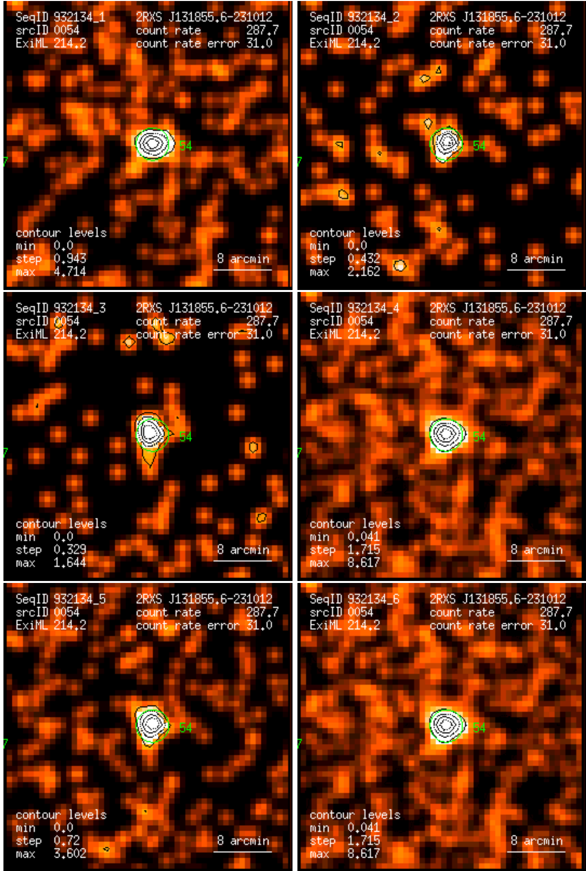
Figure 54: RASS 932134: detection 0054: band rate images, Gaussian filter: (1) PSPC channels 11 – 41, (2) 52 – 90, (3) 91 – 201, (4) 11 – 235, (5) 52 – 201, (6) 11 – 201. Broad band rates in counts/ks. Band rate contour levels in counts/ks/arcmin 2 .
