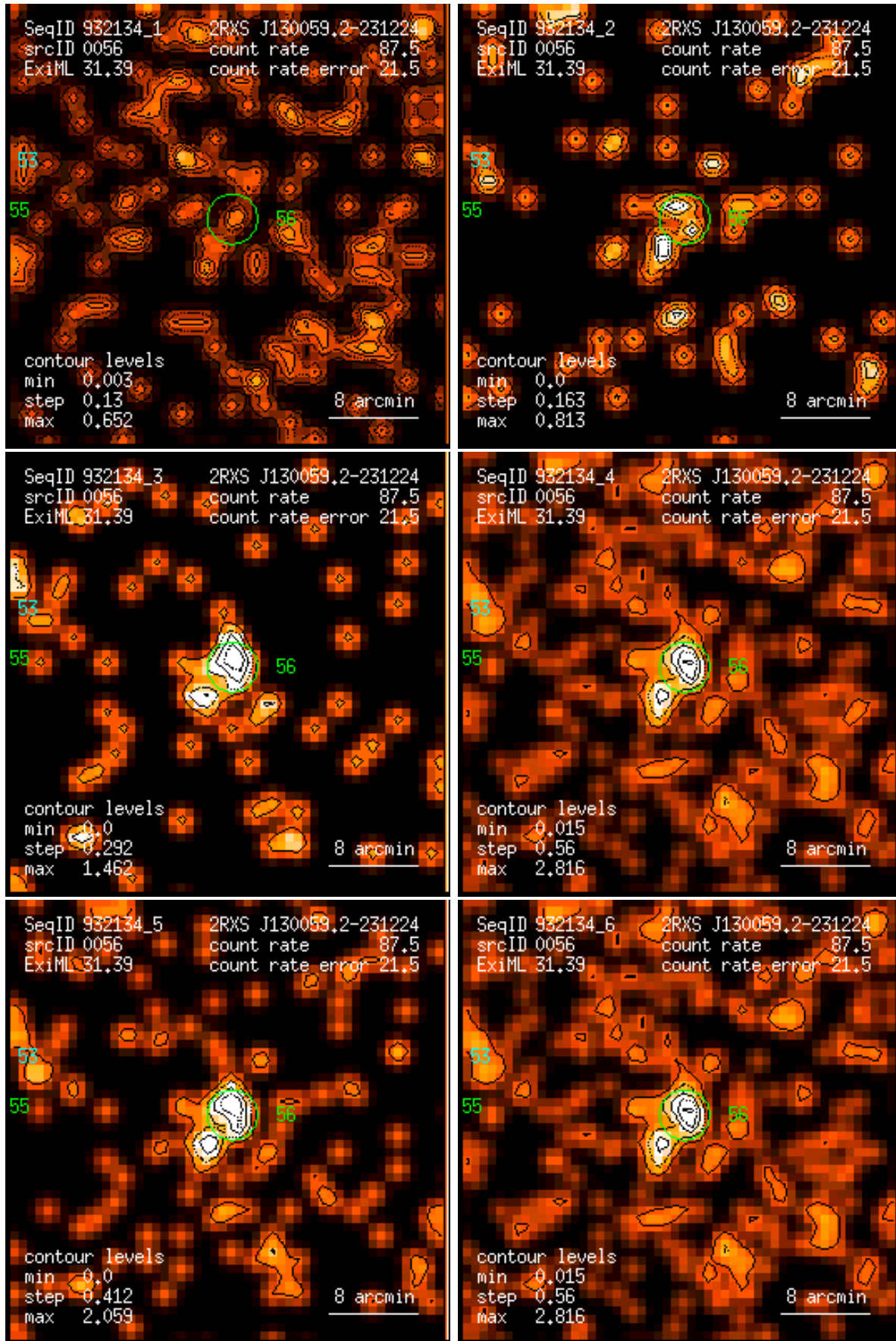
Figure 56: RASS 932134: detection 0056: band rate images, Gaussian filter: (1) PSPC channels 11 – 41, (2) 52 – 90, (3) 91 – 201, (4) 11 – 235, (5) 52 – 201, (6) 11 – 201. Broad band rates in counts/ks. Band rate contour levels in counts/ks/arcmin 2 .
