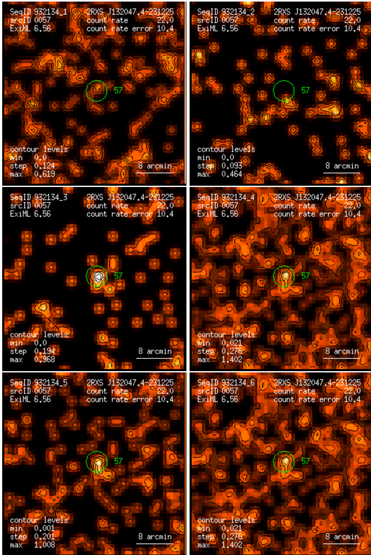
Figure 57: RASS 932134: detection 0057: band rate images, Gaussian filter: (1) PSPC channels 11 – 41, (2) 52 – 90, (3) 91 – 201, (4) 11 – 235, (5) 52 – 201, (6) 11 – 201. Broad band rates in counts/ks. Band rate contour levels in counts/ks/arcmin 2 .
