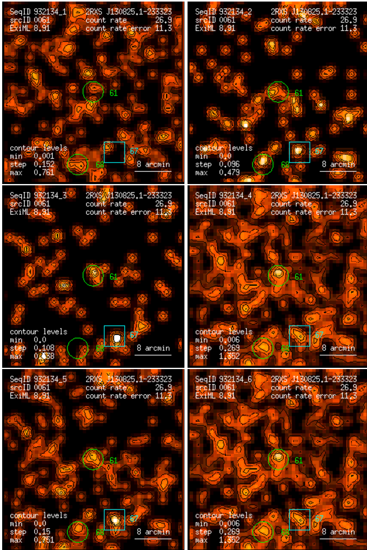
Figure 61: RASS 932134: detection 0061: band rate images, Gaussian filter: (1) PSPC channels 11 – 41, (2) 52 – 90, (3) 91 – 201, (4) 11 – 235, (5) 52 – 201, (6) 11 – 201. Broad band rates in counts/ks. Band rate contour levels in counts/ks/arcmin 2 .
