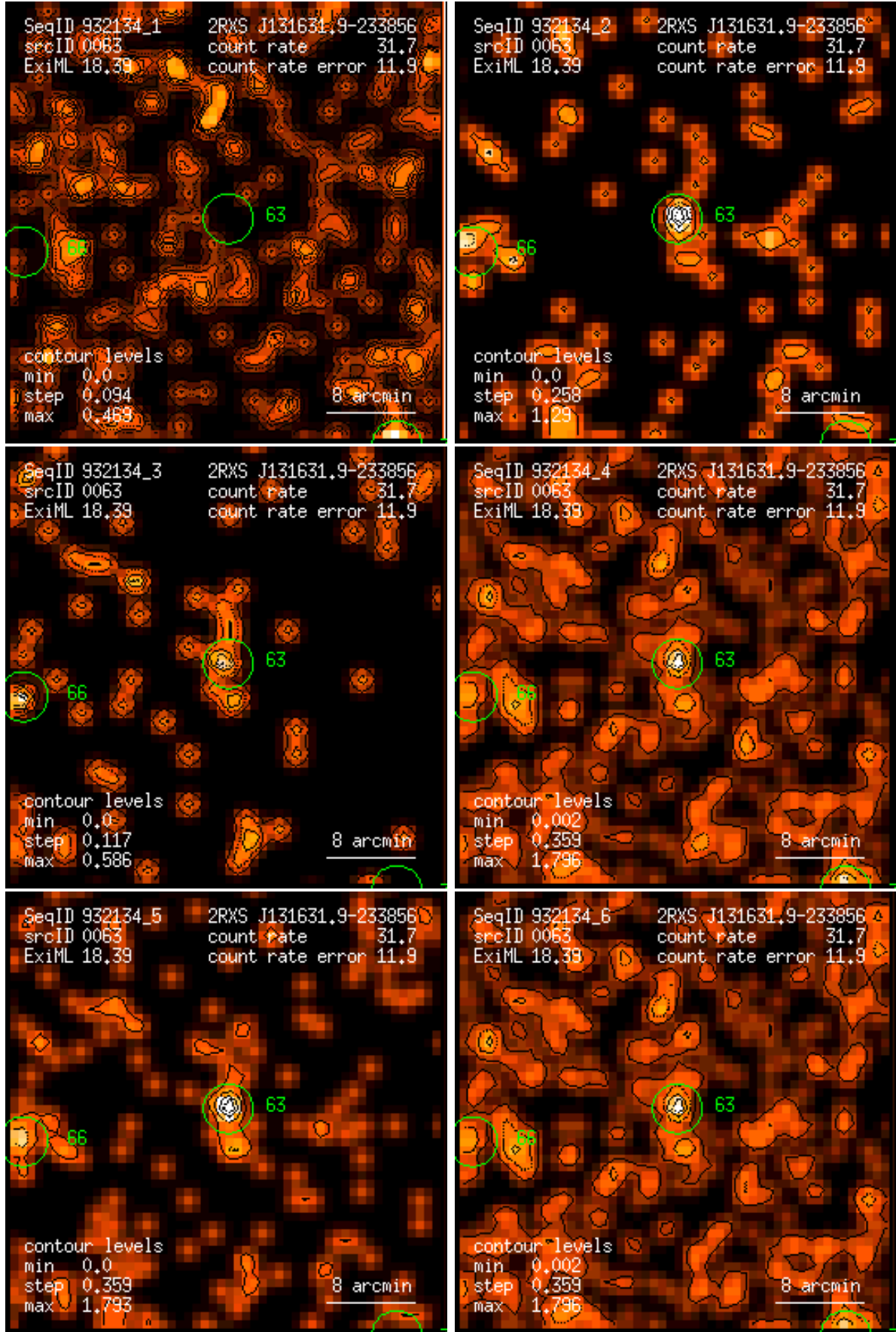
Figure 63: RASS 932134: detection 0063: band rate images, Gaussian filter: (1) PSPC channels 11 – 41, (2) 52 – 90, (3) 91 – 201, (4) 11 – 235, (5) 52 – 201, (6) 11 – 201. Broad band rates in counts/ks. Band rate contour levels in counts/ks/arcmin 2 .
