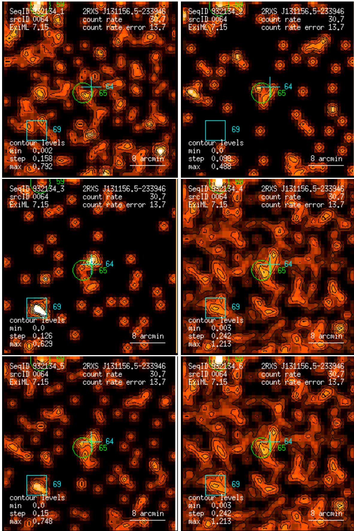
Figure 64: RASS 932134: detection 0064: band rate images, Gaussian filter: (1) PSPC channels 11 – 41, (2) 52 – 90, (3) 91 – 201, (4) 11 – 235, (5) 52 – 201, (6) 11 – 201. Broad band rates in counts/ks. Band rate contour levels in counts/ks/arcmin 2 .
