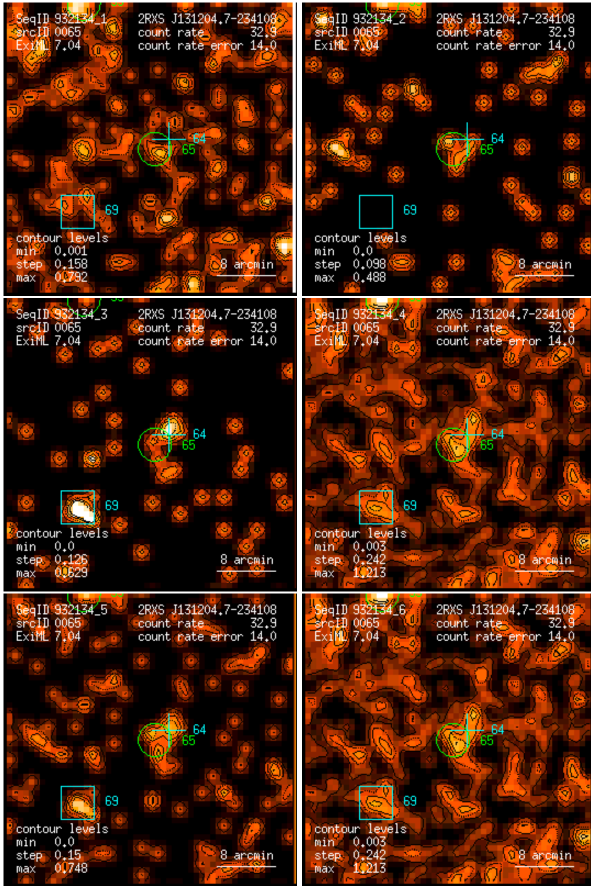
Figure 65: RASS 932134: detection 0065: band rate images, Gaussian filter: (1) PSPC channels 11 – 41, (2) 52 – 90, (3) 91 – 201, (4) 11 – 235, (5) 52 – 201, (6) 11 – 201. Broad band rates in counts/ks. Band rate contour levels in counts/ks/arcmin 2 .
