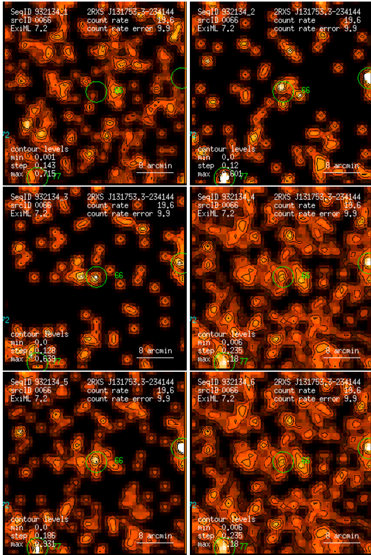
Figure 66: RASS 932134: detection 0066: band rate images, Gaussian filter: (1) PSPC channels 11 – 41, (2) 52 – 90, (3) 91 – 201, (4) 11 – 235, (5) 52 – 201, (6) 11 – 201. Broad band rates in counts/ks. Band rate contour levels in counts/ks/arcmin 2 .
