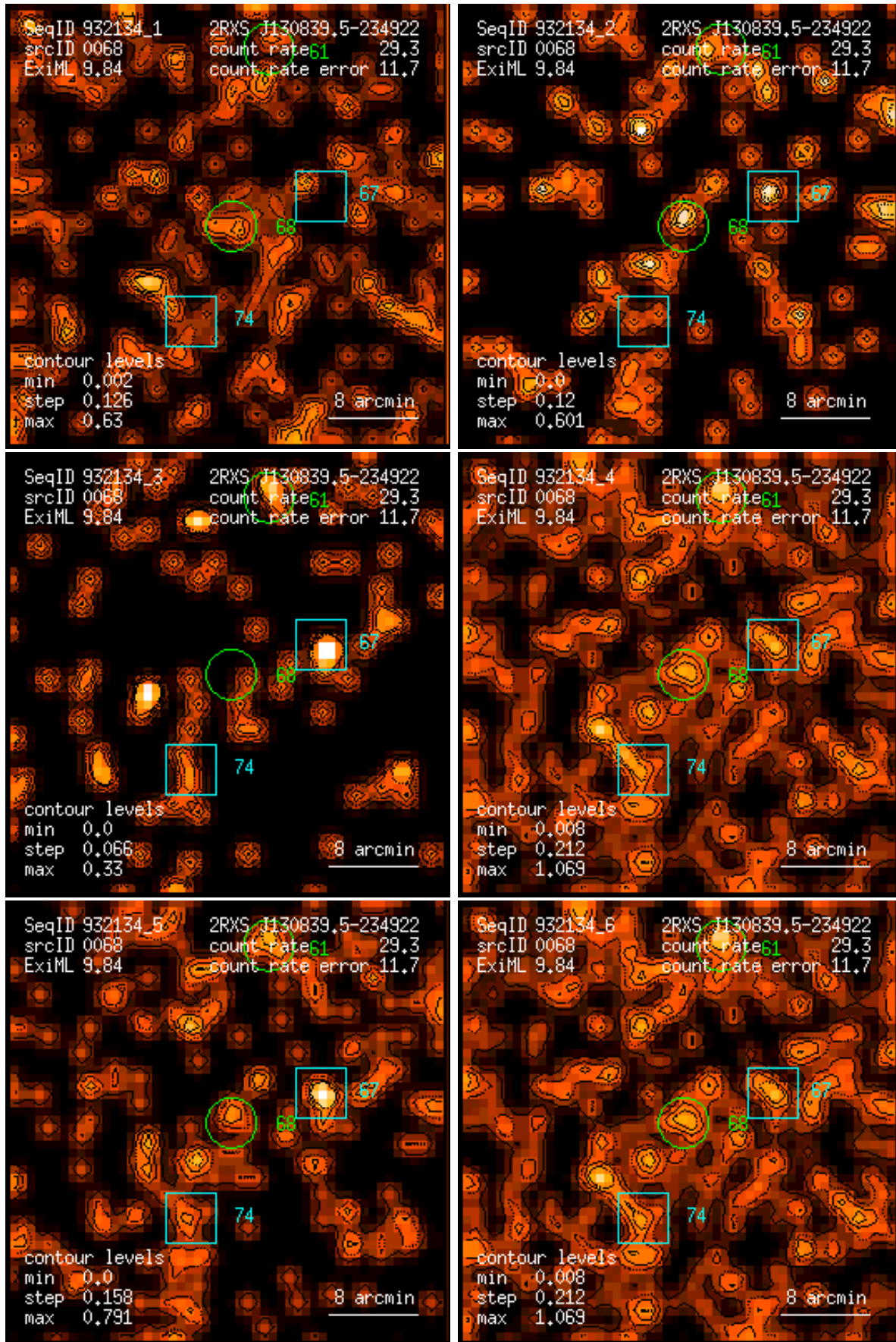
Figure 68: RASS 932134: detection 0068: band rate images, Gaussian filter: (1) PSPC channels 11 – 41, (2) 52 – 90, (3) 91 – 201, (4) 11 – 235, (5) 52 – 201, (6) 11 – 201. Broad band rates in counts/ks. Band rate contour levels in counts/ks/arcmin 2 .
