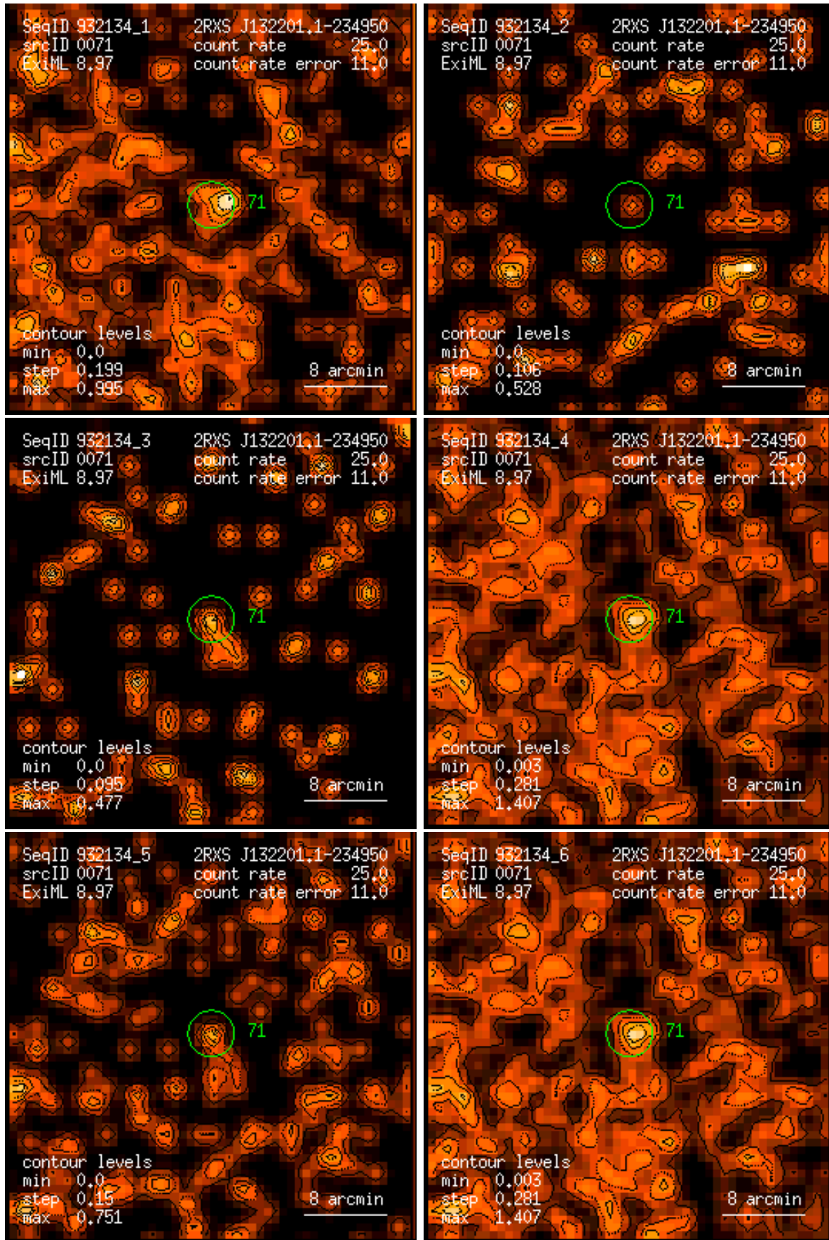
Figure 71: RASS 932134: detection 0071: band rate images, Gaussian filter: (1) PSPC channels 11 – 41, (2) 52 – 90, (3) 91 – 201, (4) 11 – 235, (5) 52 – 201, (6) 11 – 201. Broad band rates in counts/ks. Band rate contour levels in counts/ks/arcmin 2 .
