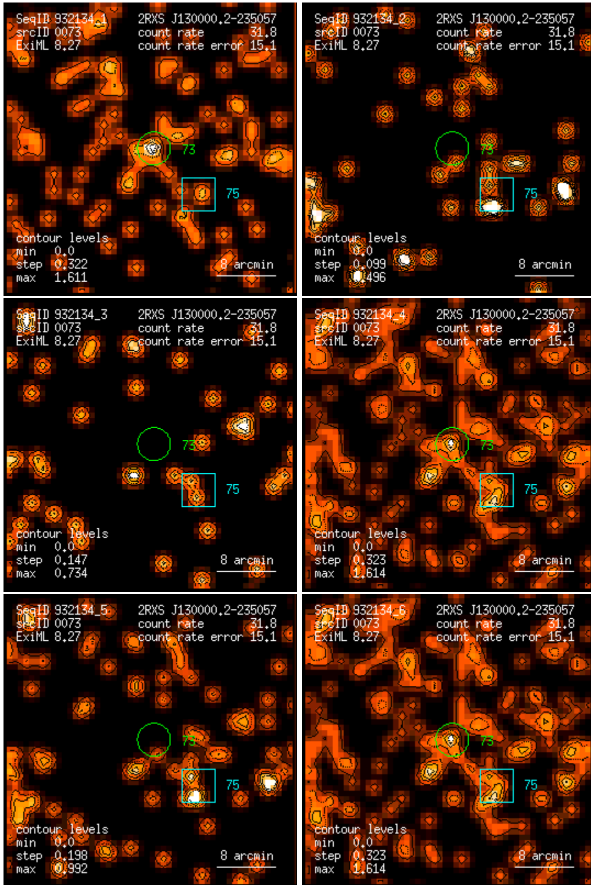
Figure 73: RASS 932134: detection 0073: band rate images, Gaussian filter: (1) PSPC channels 11 – 41, (2) 52 – 90, (3) 91 – 201, (4) 11 – 235, (5) 52 – 201, (6) 11 – 201. Broad band rates in counts/ks. Band rate contour levels in counts/ks/arcmin 2 .
