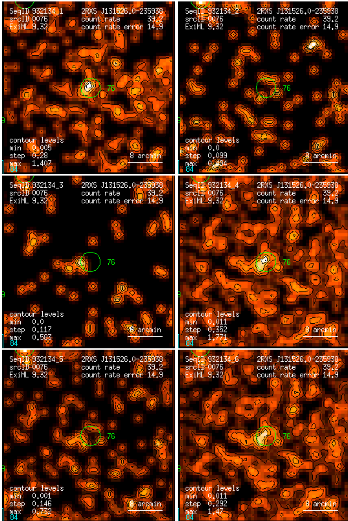
Figure 76: RASS 932134: detection 0076: band rate images, Gaussian filter: (1) PSPC channels 11 – 41, (2) 52 – 90, (3) 91 – 201, (4) 11 – 235, (5) 52 – 201, (6) 11 – 201. Broad band rates in counts/ks. Band rate contour levels in counts/ks/arcmin 2 .
