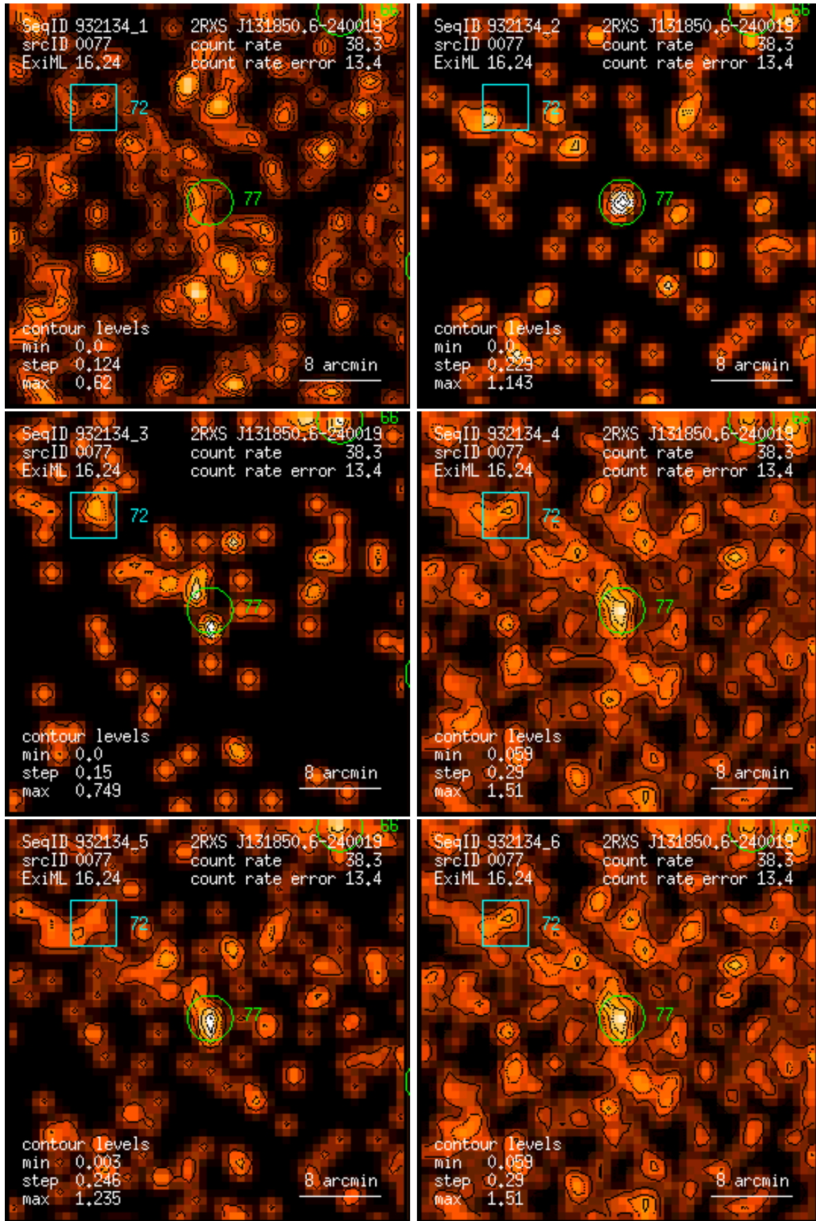
Figure 77: RASS 932134: detection 0077: band rate images, Gaussian filter: (1) PSPC channels 11 – 41, (2) 52 – 90, (3) 91 – 201, (4) 11 – 235, (5) 52 – 201, (6) 11 – 201. Broad band rates in counts/ks. Band rate contour levels in counts/ks/arcmin 2 .
