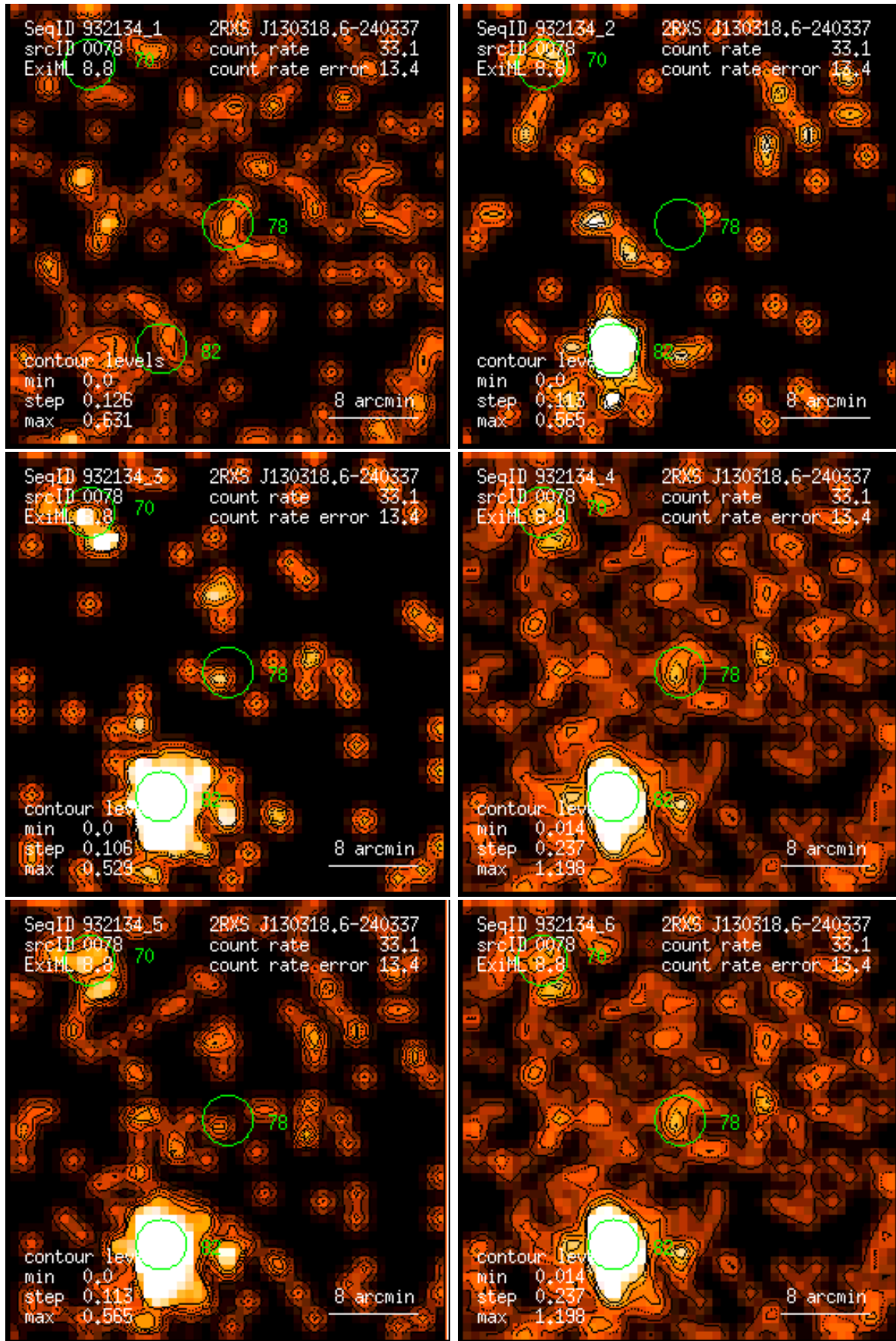
Figure 78: RASS 932134: detection 0078: band rate images, Gaussian filter: (1) PSPC channels 11 – 41, (2) 52 – 90, (3) 91 – 201, (4) 11 – 235, (5) 52 – 201, (6) 11 – 201. Broad band rates in counts/ks. Band rate contour levels in counts/ks/arcmin 2 .
