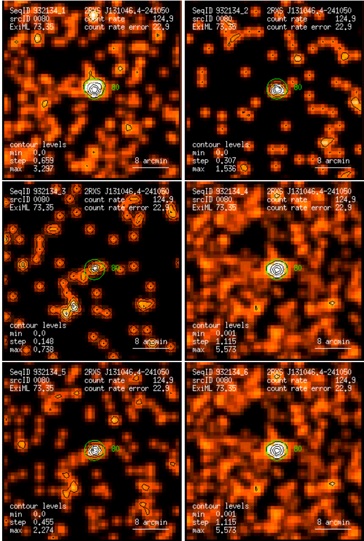
Figure 80: RASS 932134: detection 0080: band rate images, Gaussian filter: (1) PSPC channels 11 – 41, (2) 52 – 90, (3) 91 – 201, (4) 11 – 235, (5) 52 – 201, (6) 11 – 201. Broad band rates in counts/ks. Band rate contour levels in counts/ks/arcmin 2 .
