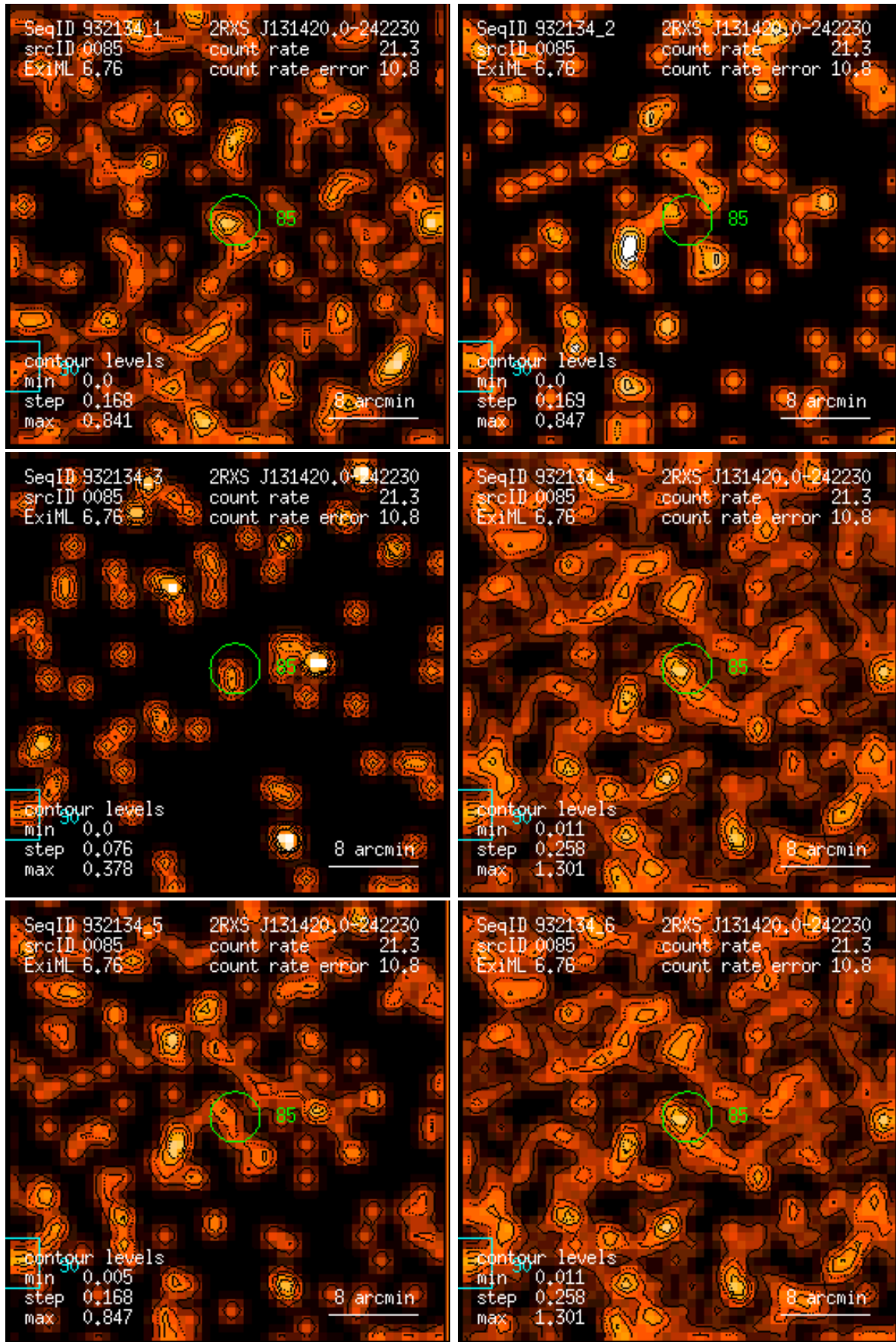
Figure 85: RASS 932134: detection 0085: band rate images, Gaussian filter: (1) PSPC channels 11 – 41, (2) 52 – 90, (3) 91 – 201, (4) 11 – 235, (5) 52 – 201, (6) 11 – 201. Broad band rates in counts/ks. Band rate contour levels in counts/ks/arcmin 2 .
