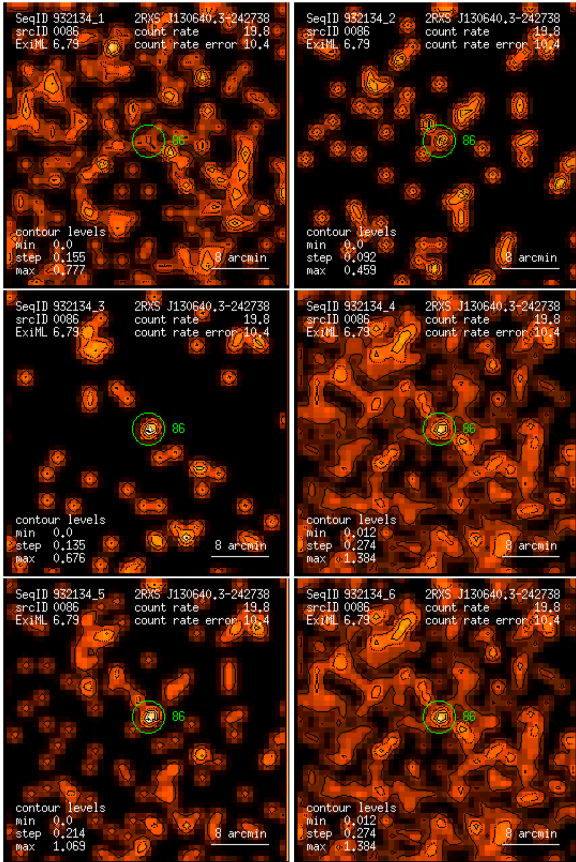
Figure 86: RASS 932134: detection 0086: band rate images, Gaussian filter: (1) PSPC channels 11 – 41, (2) 52 – 90, (3) 91 – 201, (4) 11 – 235, (5) 52 – 201, (6) 11 – 201. Broad band rates in counts/ks. Band rate contour levels in counts/ks/arcmin 2 .
